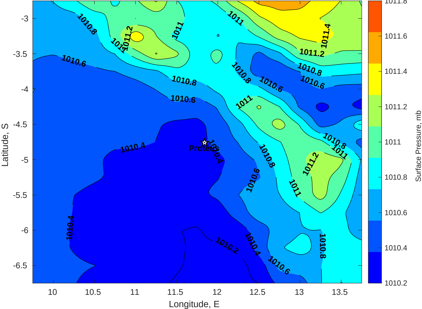
Surface Pressure (mb) for Proteus at 19-May-2025 00:00:00
