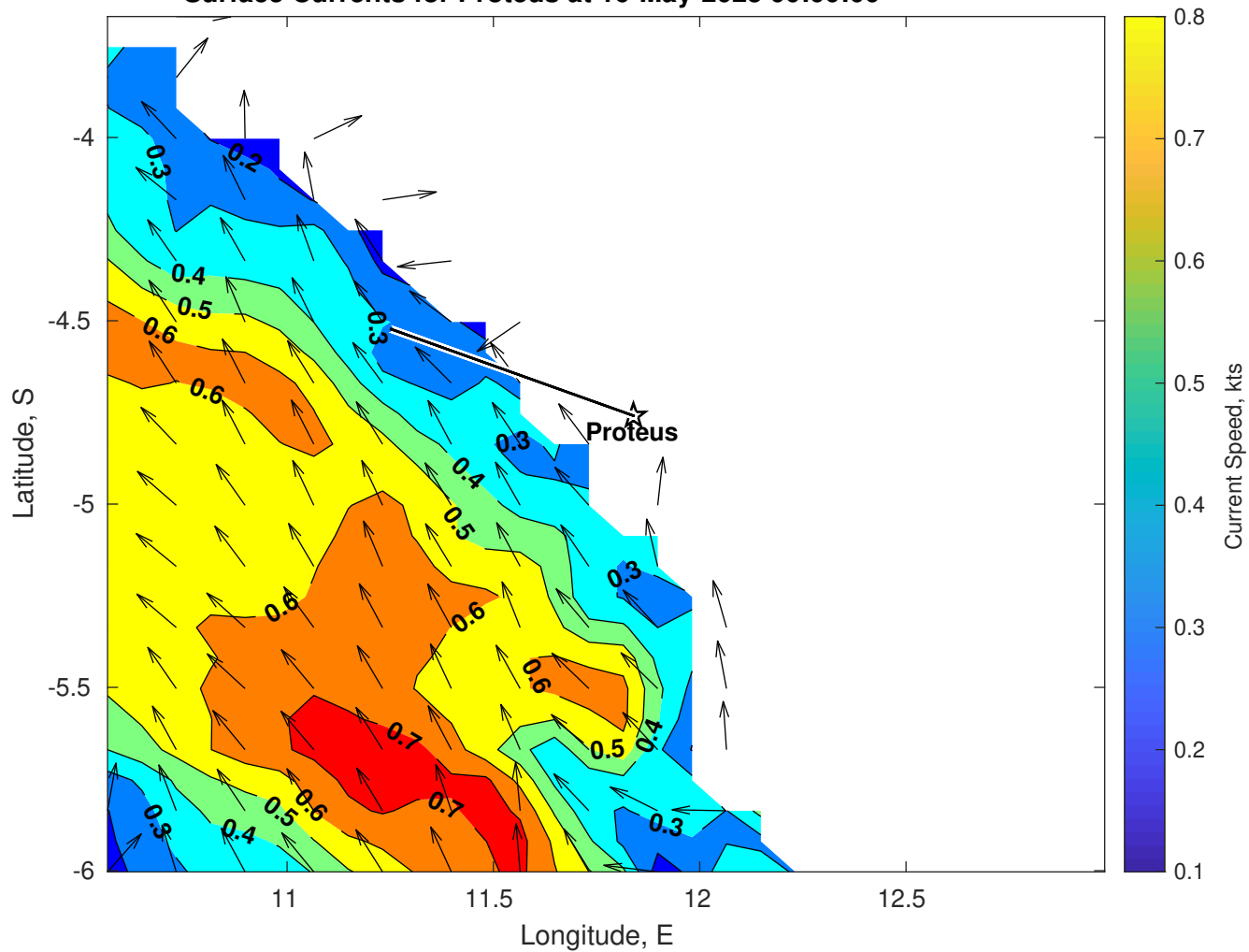
Surface Currents for Proteus at 16-May-2025 00:00:00
