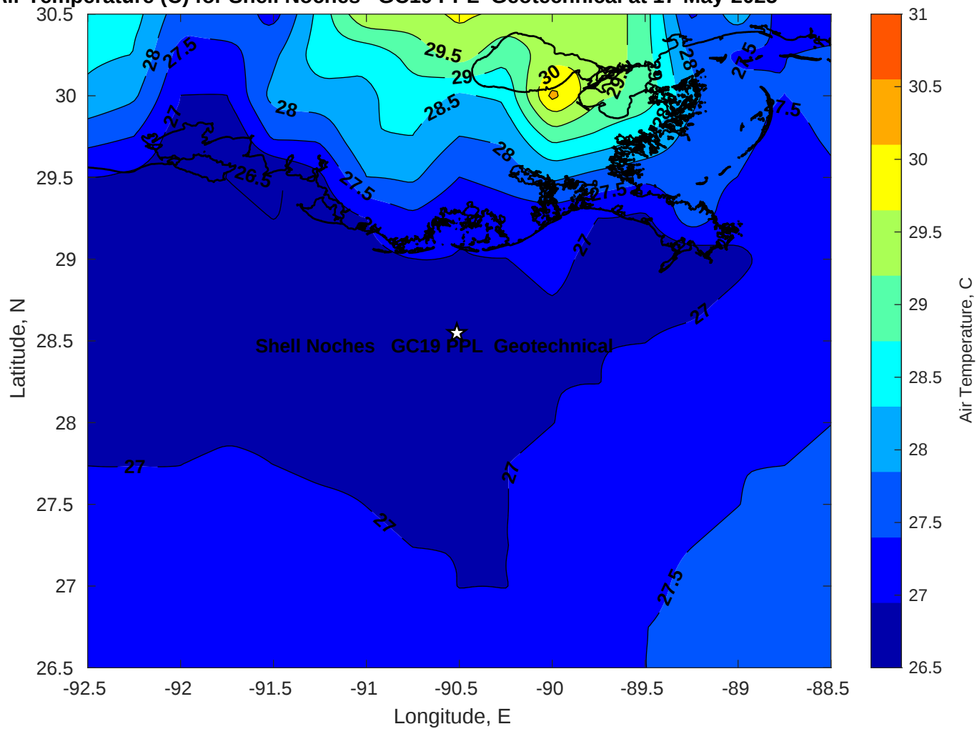
Air Temperature (C) for Shell Noches GC19 PPL Geotechnical at 17-May-2025
