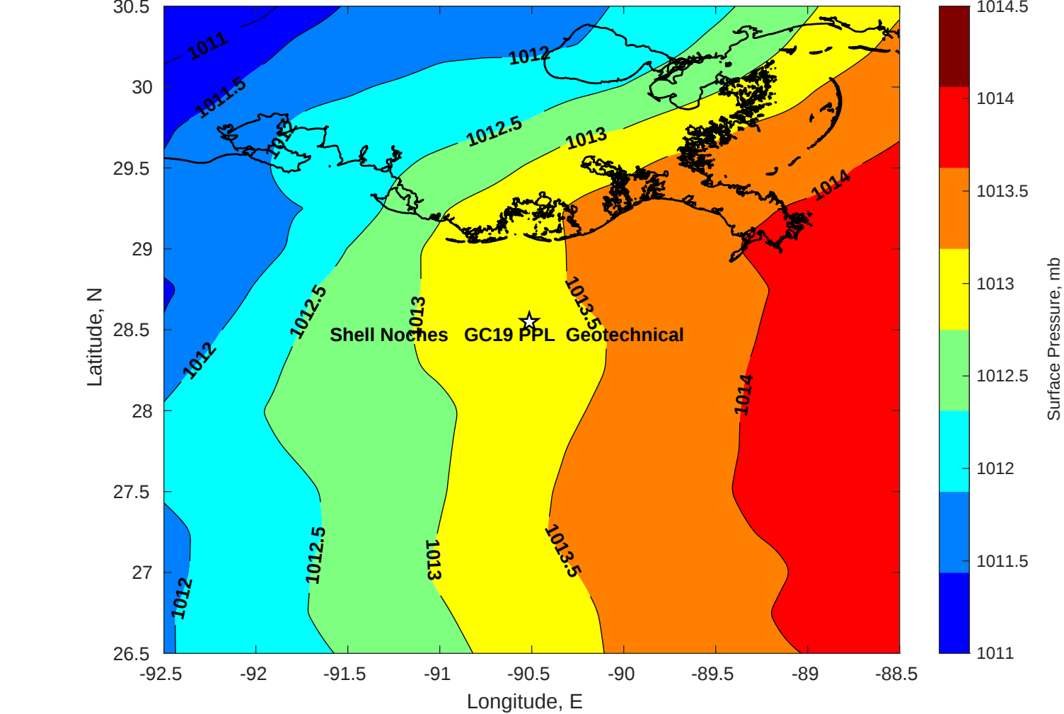
Surface Pressure (mb) for Shell Noches GC19 PPL Geotechnical at 17-May-2025 00:00:00
