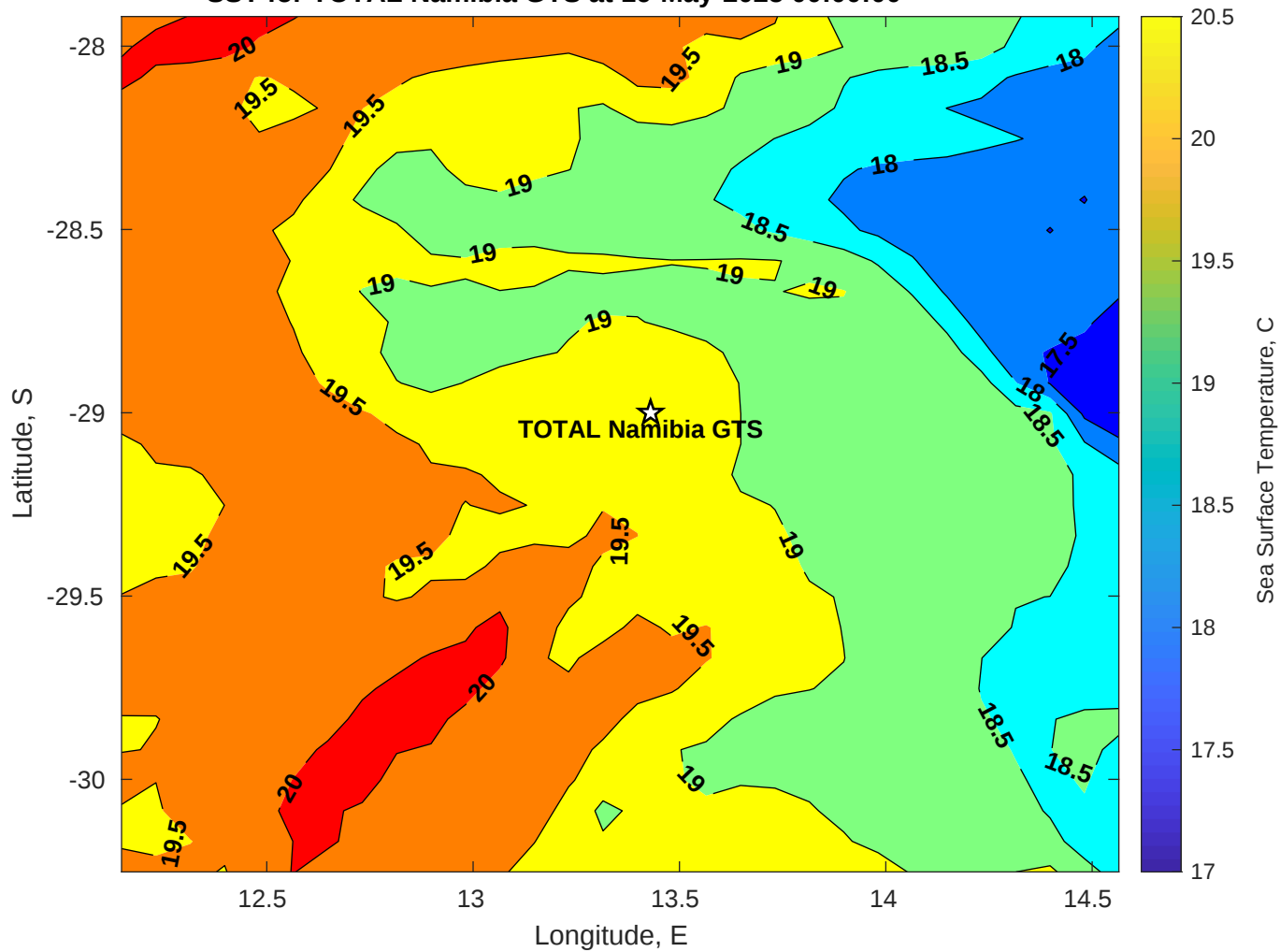
SST for TOTAL Namibia GTS at 16-May-2025 00:00:00
