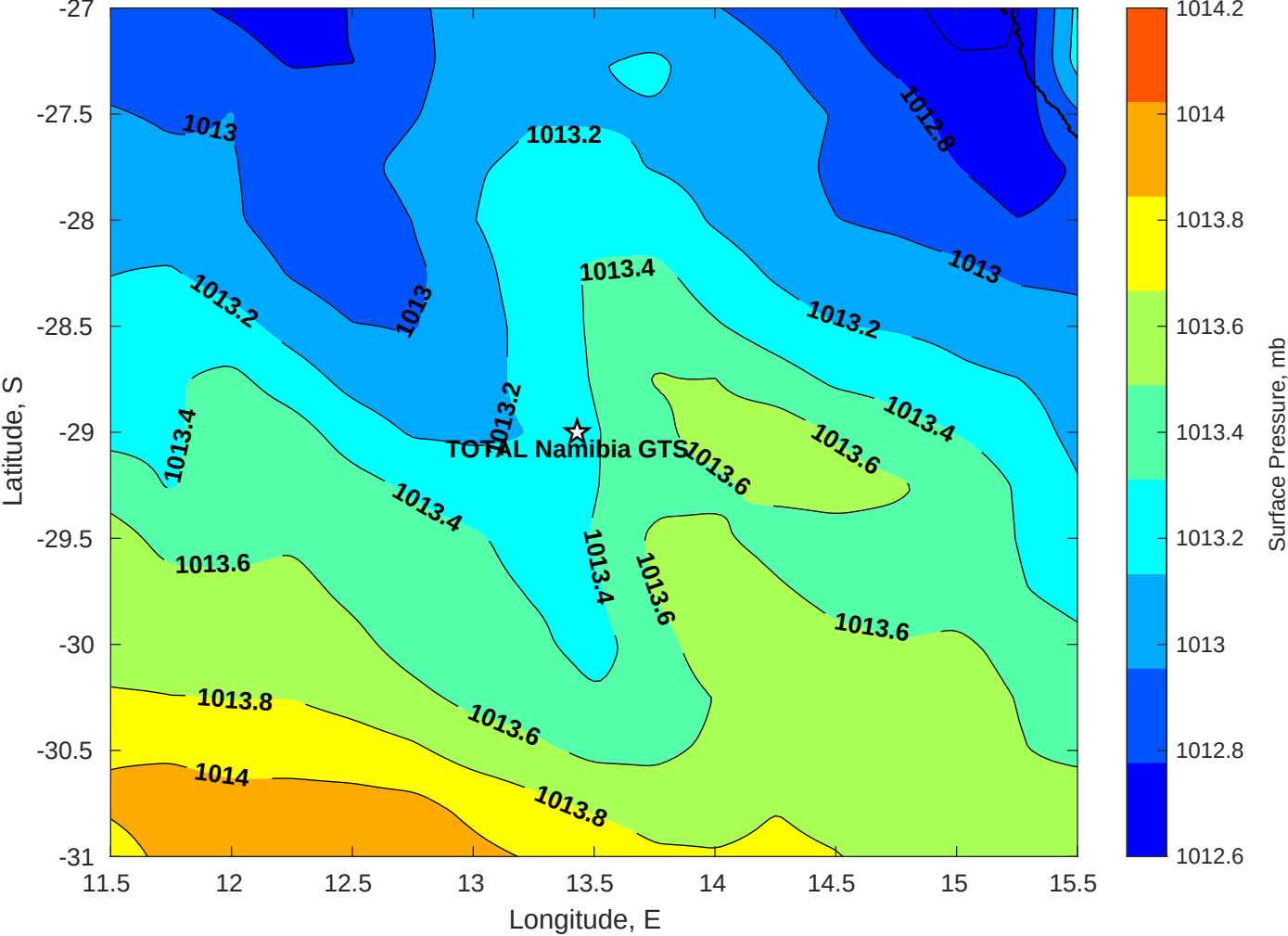
Surface Pressure (mb) for TOTAL Namibia GTS at 17-May-2025 00:00:00
