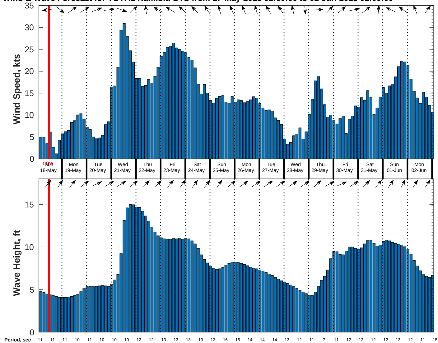
Wind & Wave Forecast for TOTAL Namibia GTS from 17-May-2025 02:00:00 to 02-Jun-2025 02:00:00
