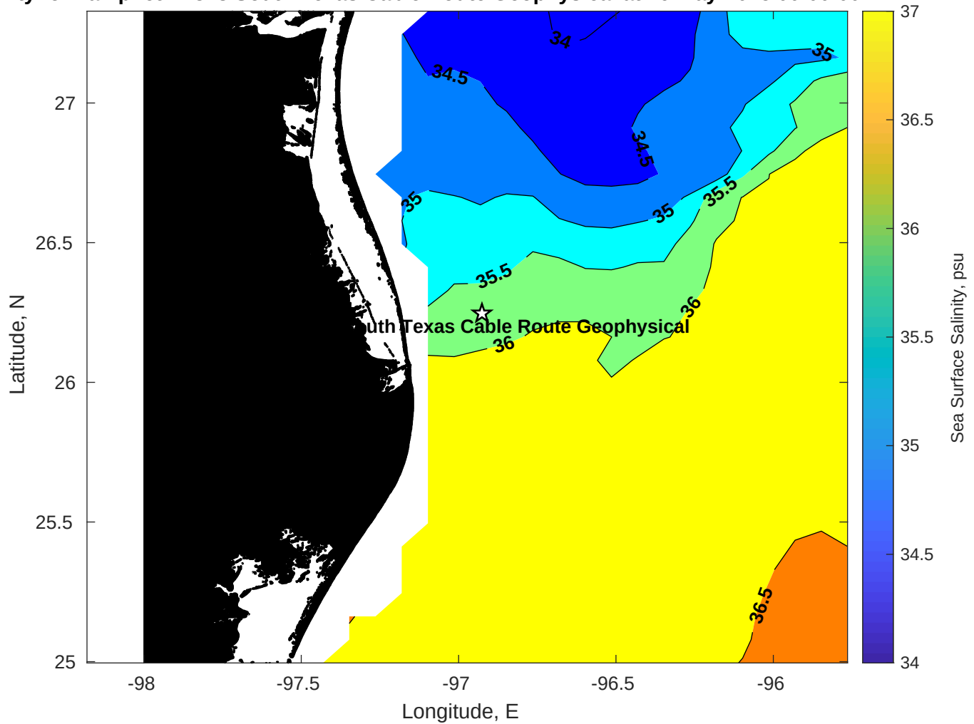
Surface Salinity for Tampnet P2378 South Texas Cable Route Geophysical at 16-May-2025 00:00:00
