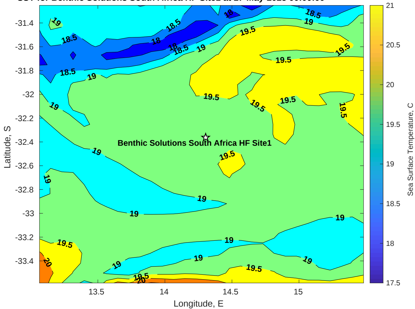
SST for Benthic Solutions South Africa HF Site1 at 17-May-2025 00:00:00
