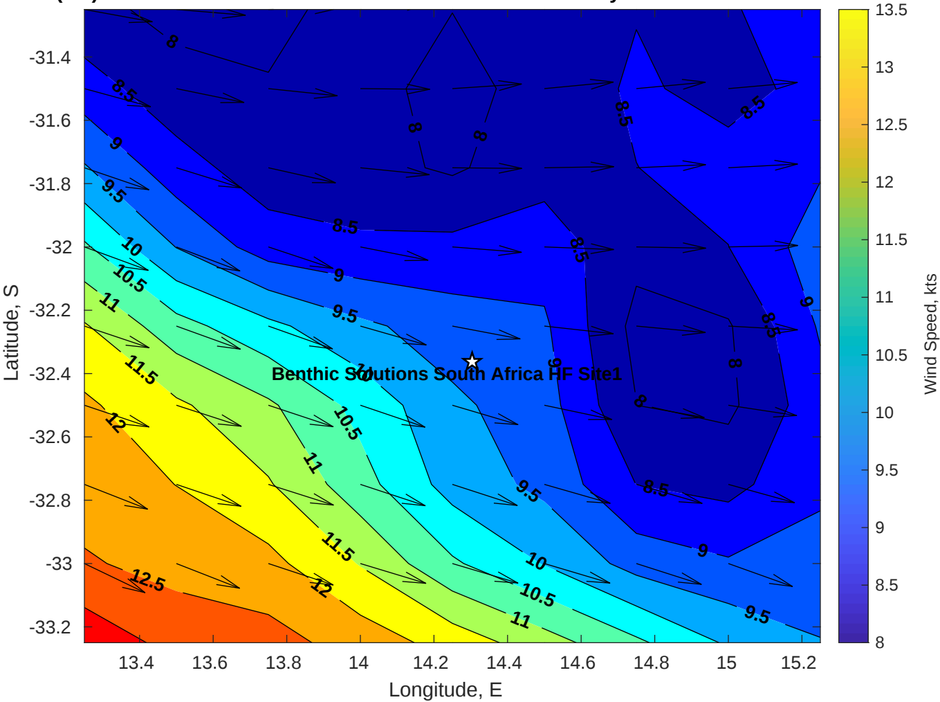
Winds (kts) for Benthic Solutions South Africa HF Site1 at 18-May-2025 09:00:00
