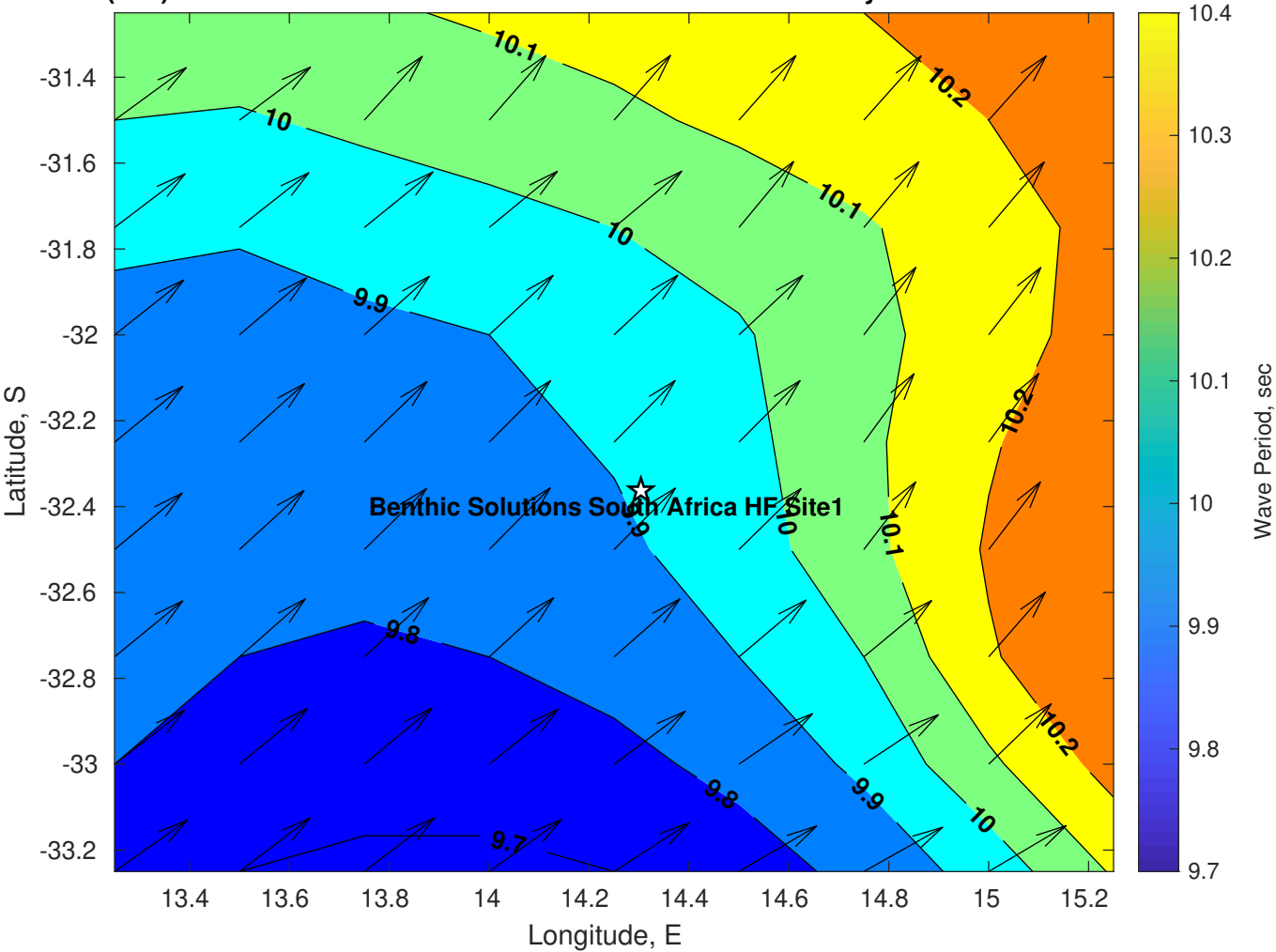
Wave Period (sec) for Benthic Solutions South Africa HF Site1 at 18-May-2025 09:00:00
