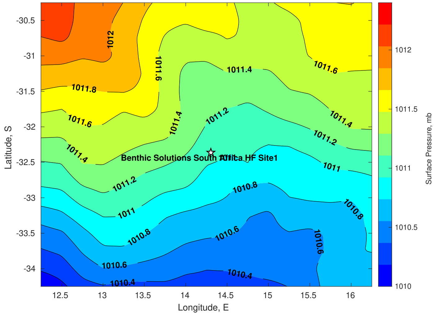
Surface Pressure (mb) for Benthic Solutions South Africa HF Site1 at 18-May-2025 00:00:00
