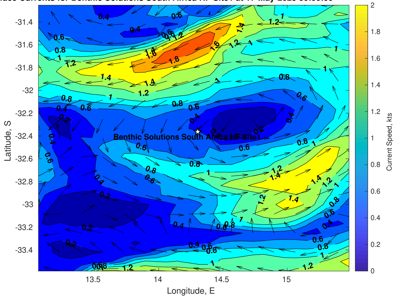
Surface Currents for Benthic Solutions South Africa HF Site1 at 17-May-2025 00:00:00
