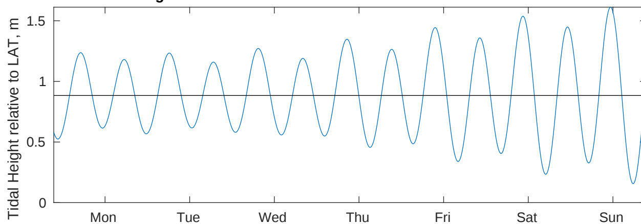
Tidal Currents and Heights for Benthic Solutions South Africa HF Site1 at 20250518
