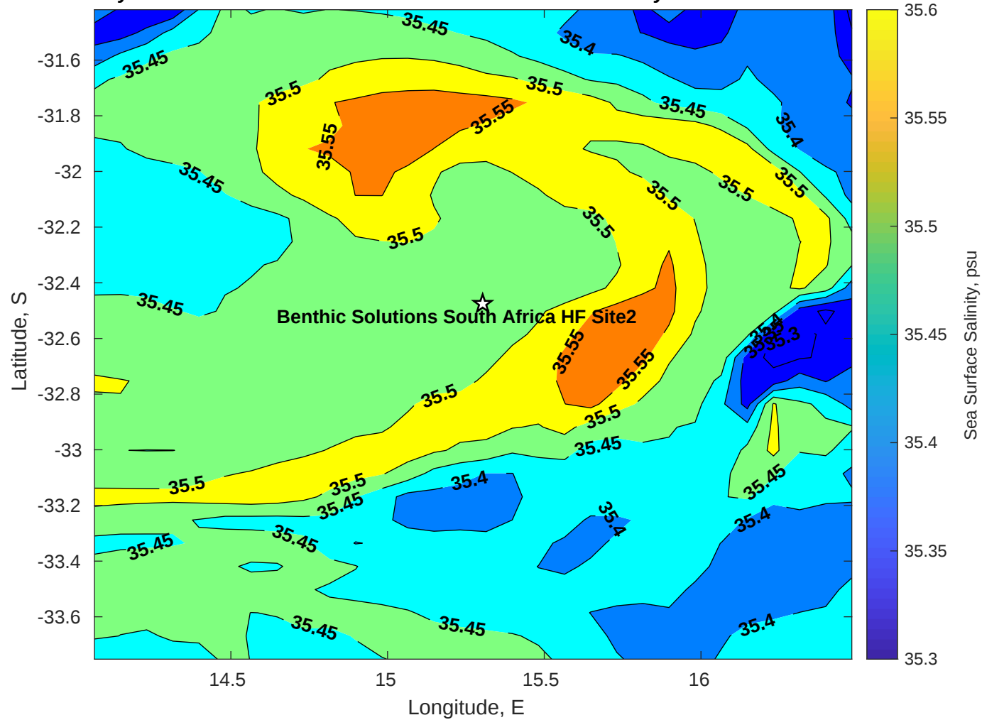
Surface Salinity for Benthic Solutions South Africa HF Site2 at 17-May-2025 00:00:00
