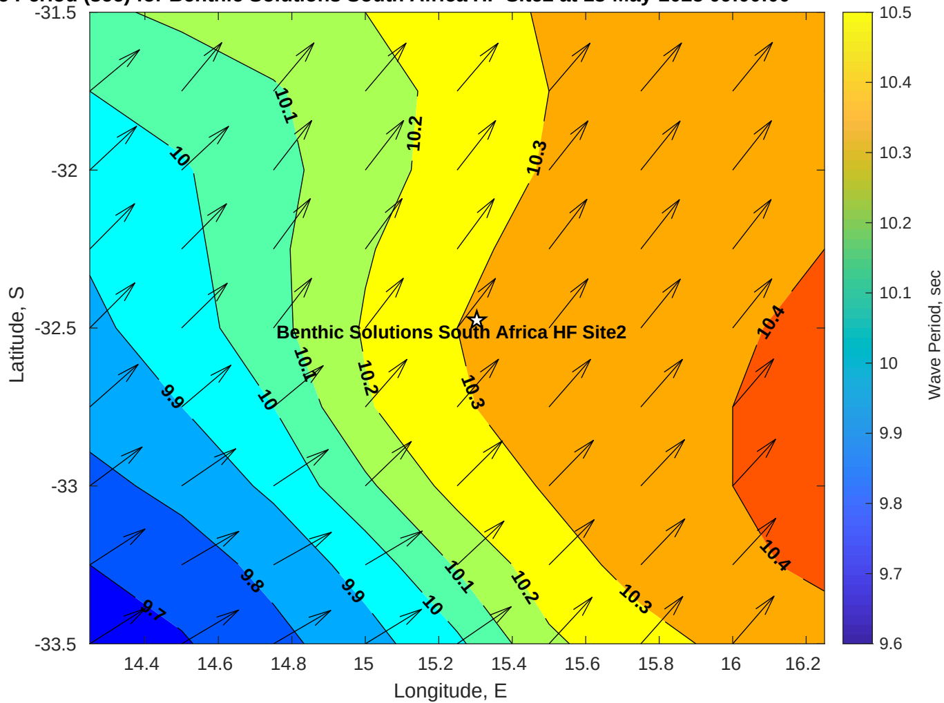
Wave Period (sec) for Benthic Solutions South Africa HF Site2 at 18-May-2025 09:00:00
