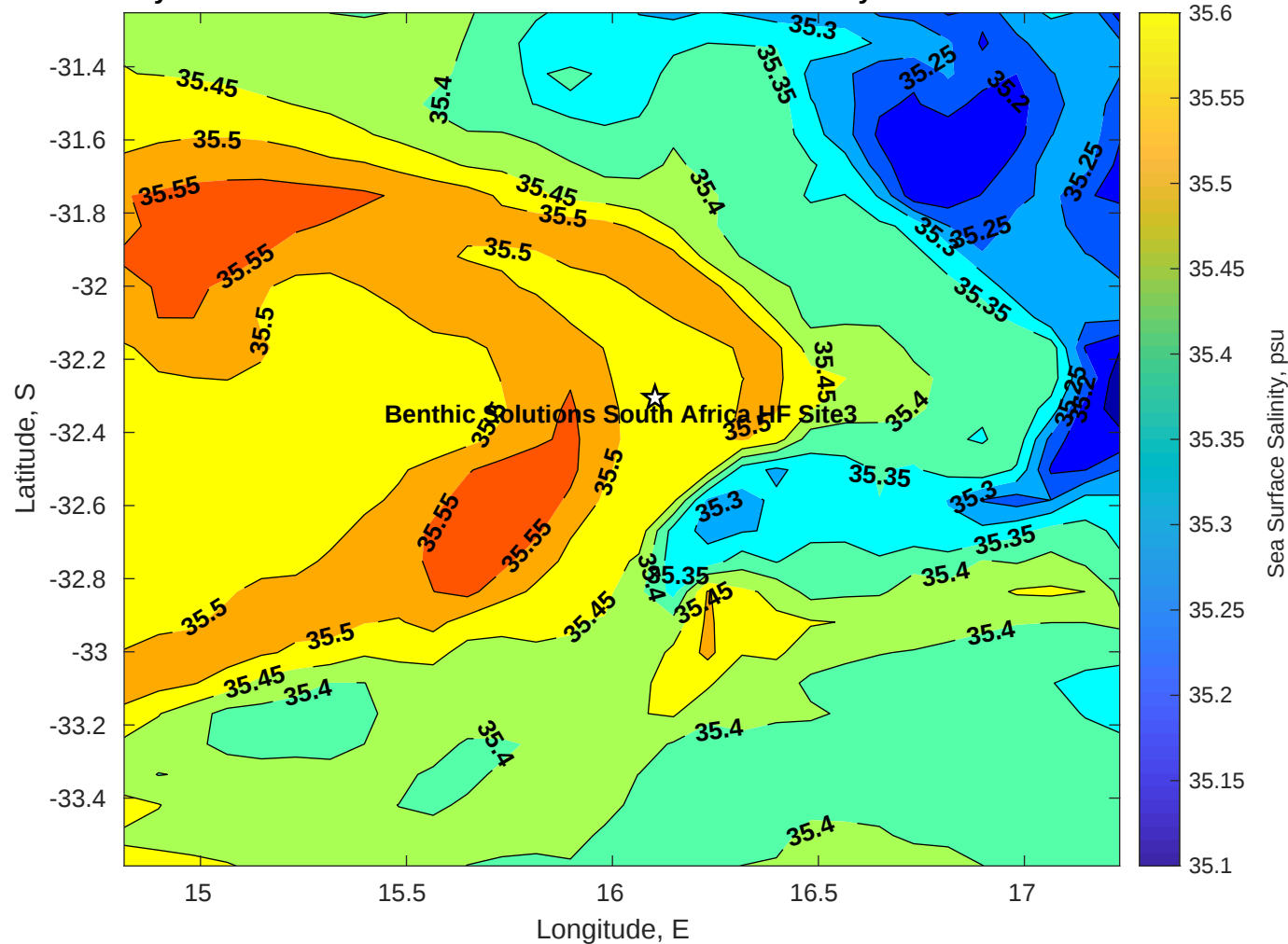
Surface Salinity for Benthic Solutions South Africa HF Site3 at 17-May-2025 00:00:00
