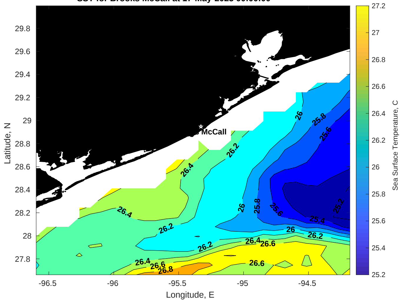
SST for Brooks McCall at 17-May-2025 00:00:00
