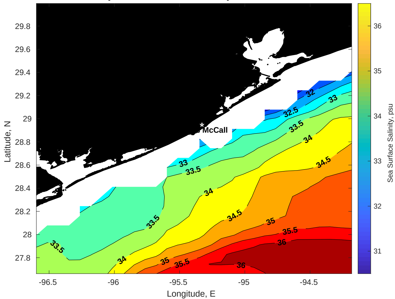
Surface Salinity for Brooks McCall at 17-May-2025 00:00:00
