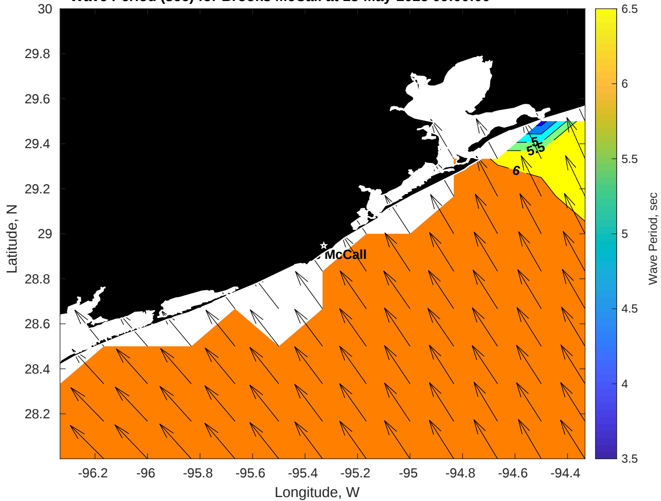
Wave Period (sec) for Brooks McCall at 18-May-2025 09:00:00
