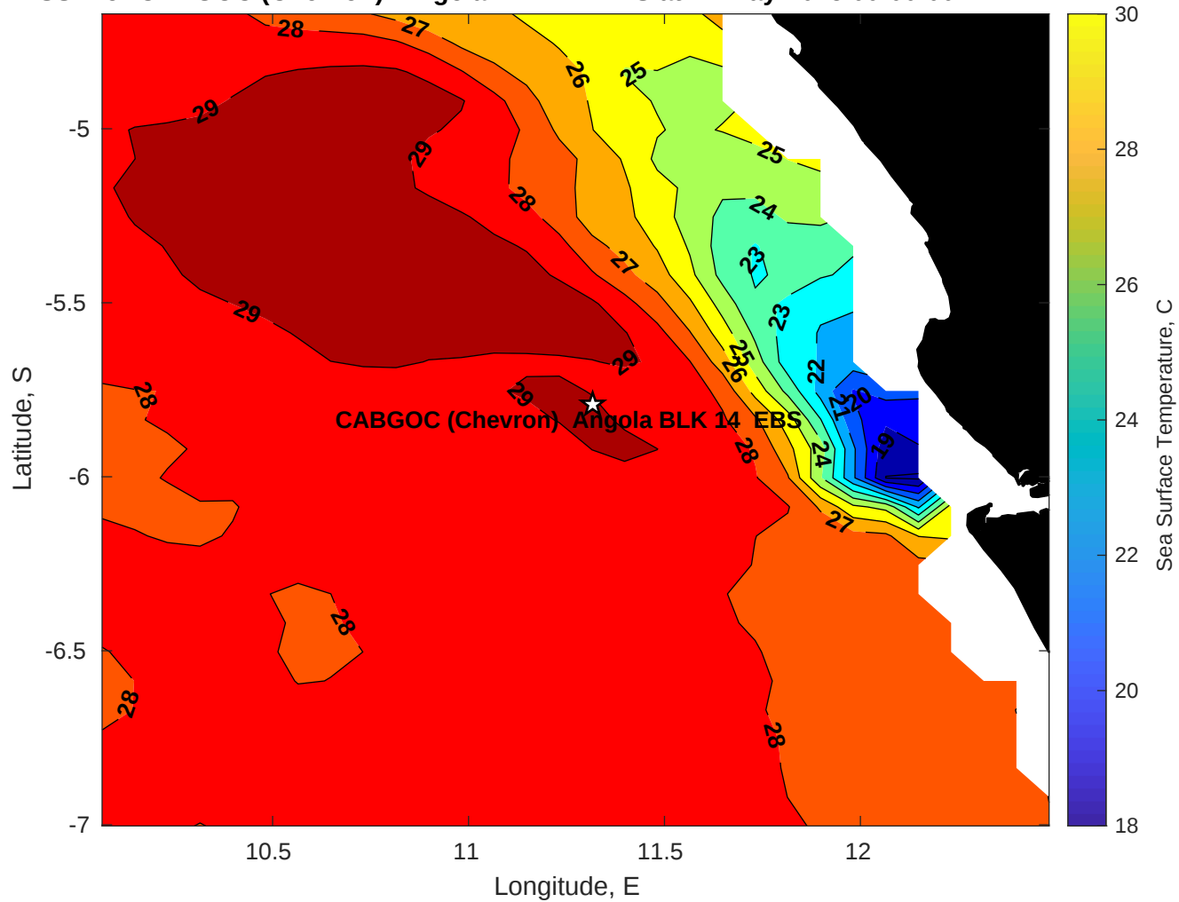
SST for CABGOC (Chevron) Angola BLK 14 EBS at 17-May-2025 00:00:00
