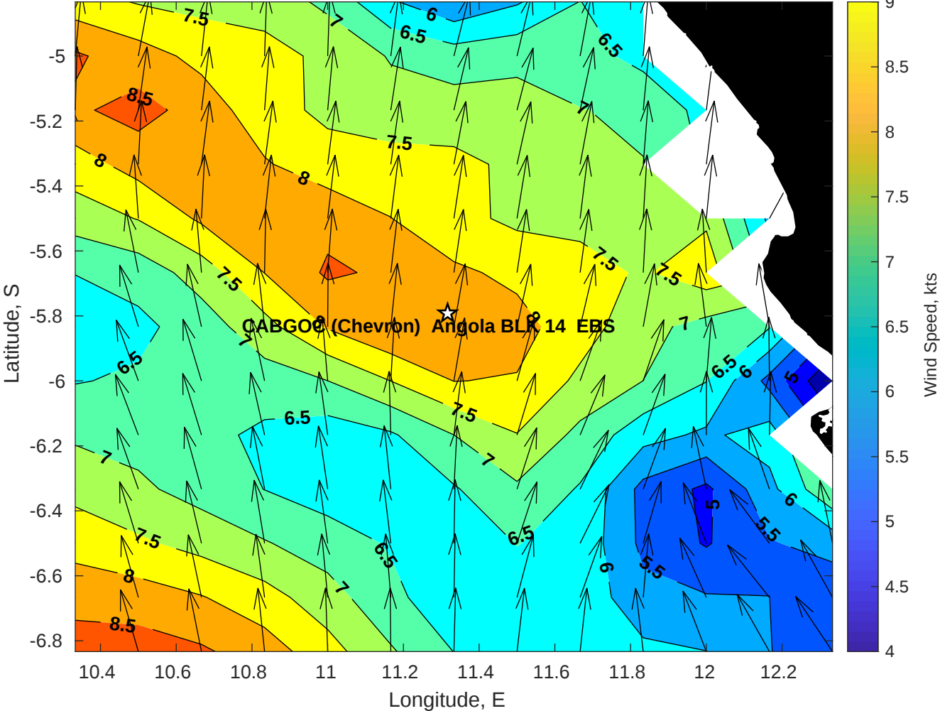
Winds (kts) for CABGOC (Chevron) Angola BLK 14 EBS at 18-May-2025 09:00:00
