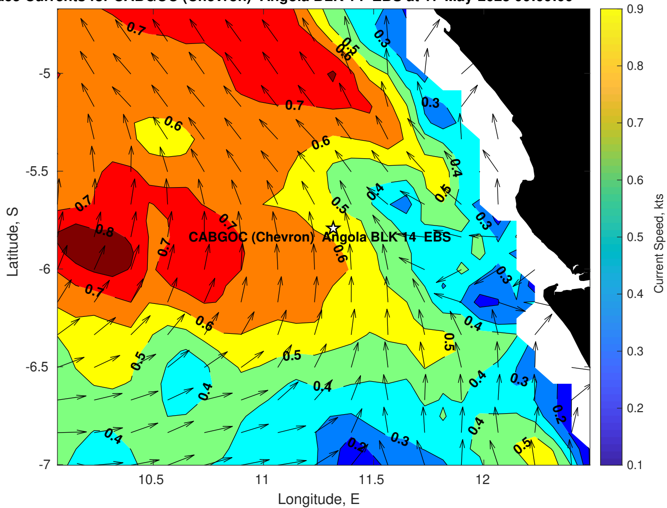
Surface Currents for CABGOC (Chevron) Angola BLK 14 EBS at 17-May-2025 00:00:00
