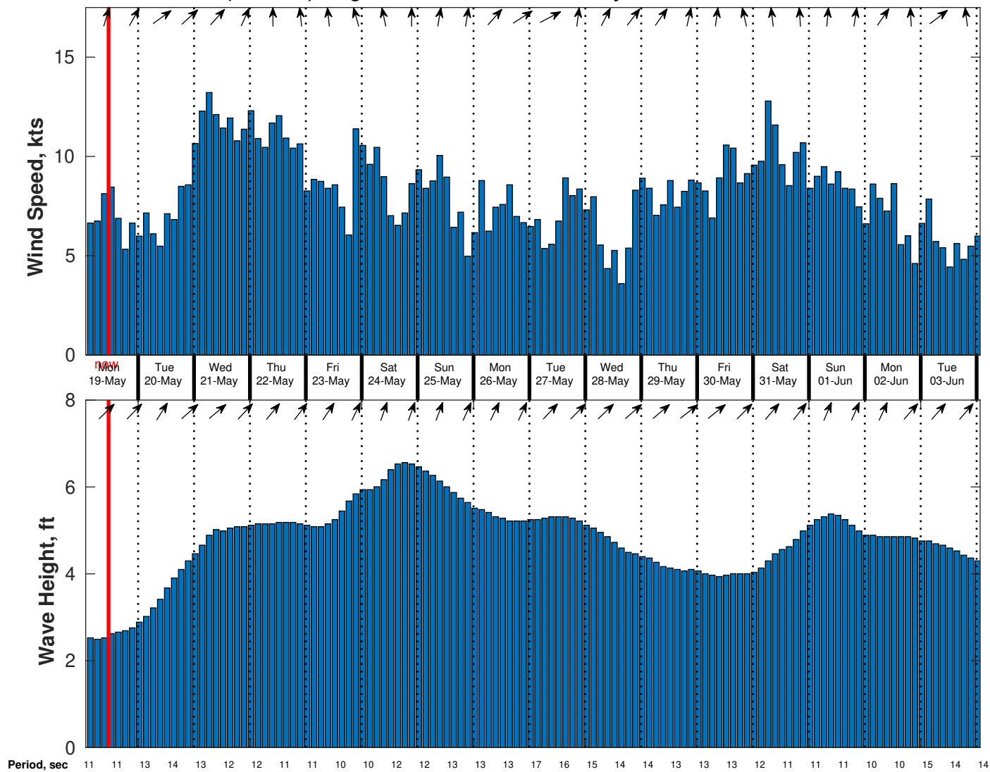
Wind & Wave Forecast for CABGOC (Chevron) Angola BLK 14 EBS from 18-May-2025 02:00:00 to 03-Jun-2025 02:00:00
