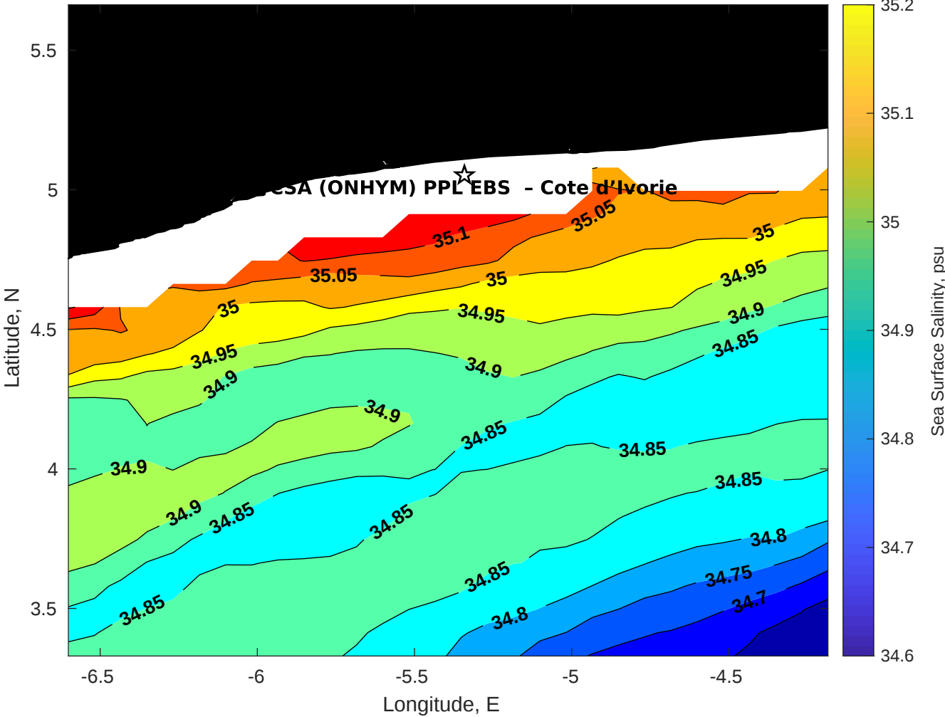
Surface Salinity for CSA (ONHYM) PPL EBS - Cote d'Ivoire at 17-May-2025 00:00:00
