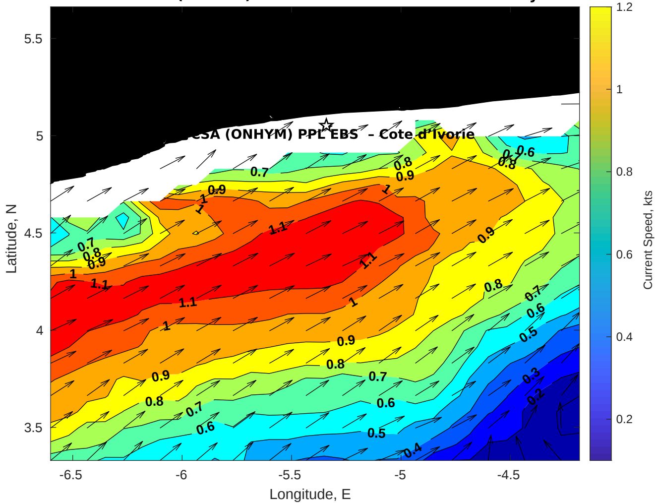
Surface Currents for CSA (ONHYM) PPL EBS - Cote d'Ivoire at 17-May-2025 00:00:00
