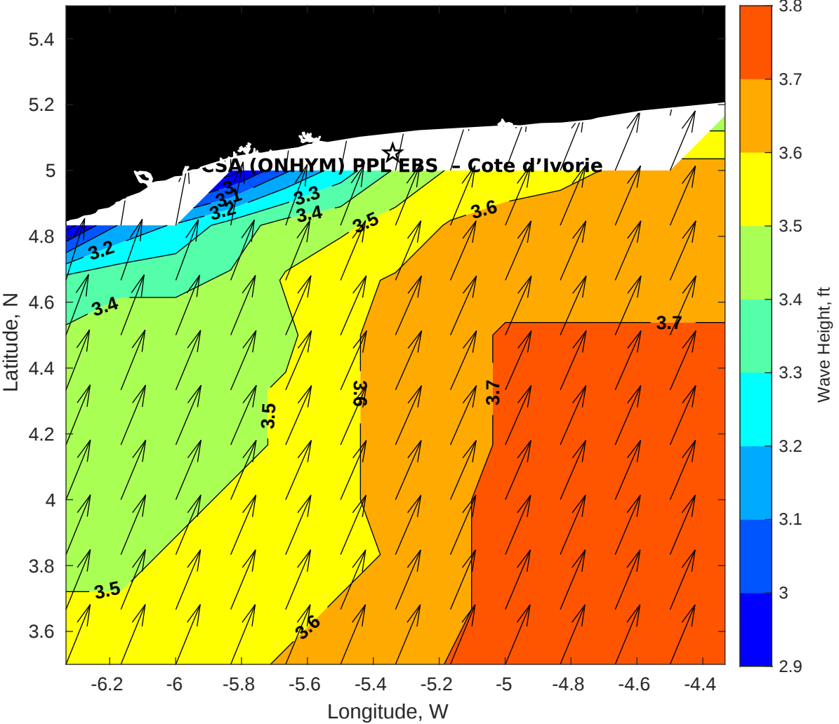
Wave Height (ft) for CSA (ONHYM) PPL EBS - Cote d'Ivoire at 18-May-2025 09:00:00
