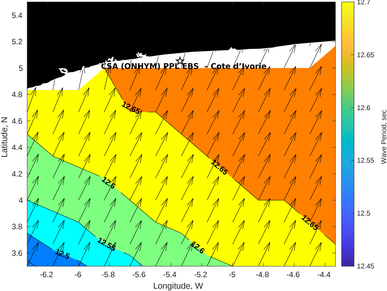
Wave Period (sec) for CSA (ONHYM) PPL EBS - Cote d'Ivoire at 18-May-2025 09:00:00
