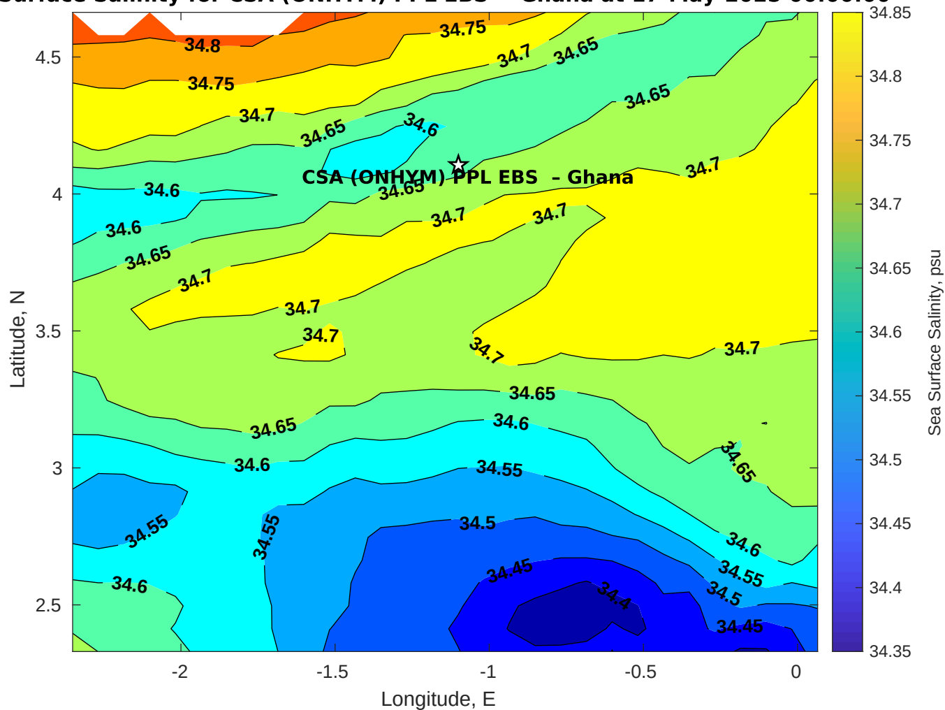
Surface Salinity for CSA (ONHYM) PPL EBS - Ghana at 17-May-2025 00:00:00
