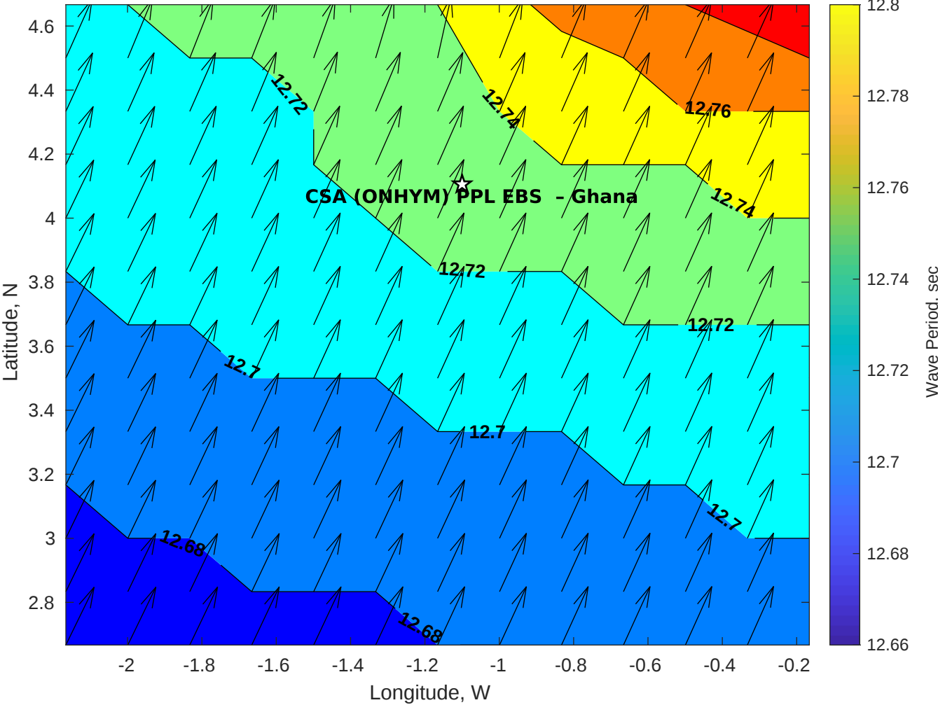
Wave Period (sec) for CSA (ONHYM) PPL EBS - Ghana at 18-May-2025 09:00:00
