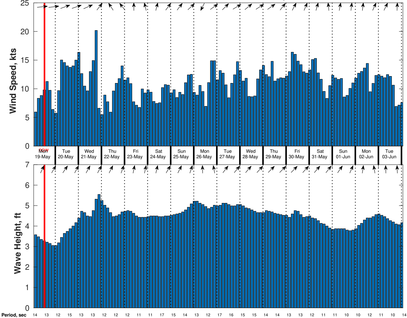
Wind & Wave Forecast for CSA (ONHYM) PPL EBS - Ghana from 18-May-2025 02:00:00 to 03-Jun-2025 02:00:00
