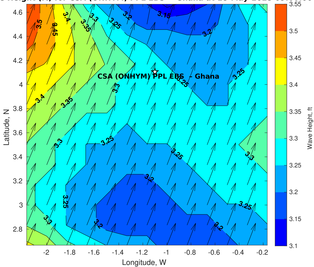
Wave Height (ft) for CSA (ONHYM) PPL EBS - Ghana at 18-May-2025 09:00:00
