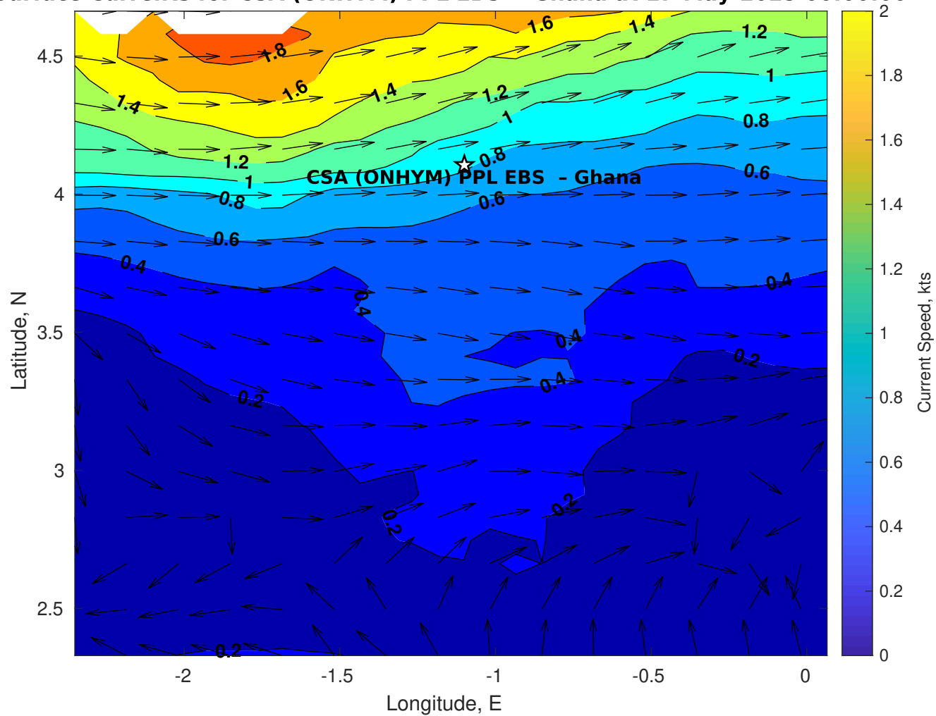
Surface Currents for CSA (ONHYM) PPL EBS - Ghana at 17-May-2025 00:00:00
