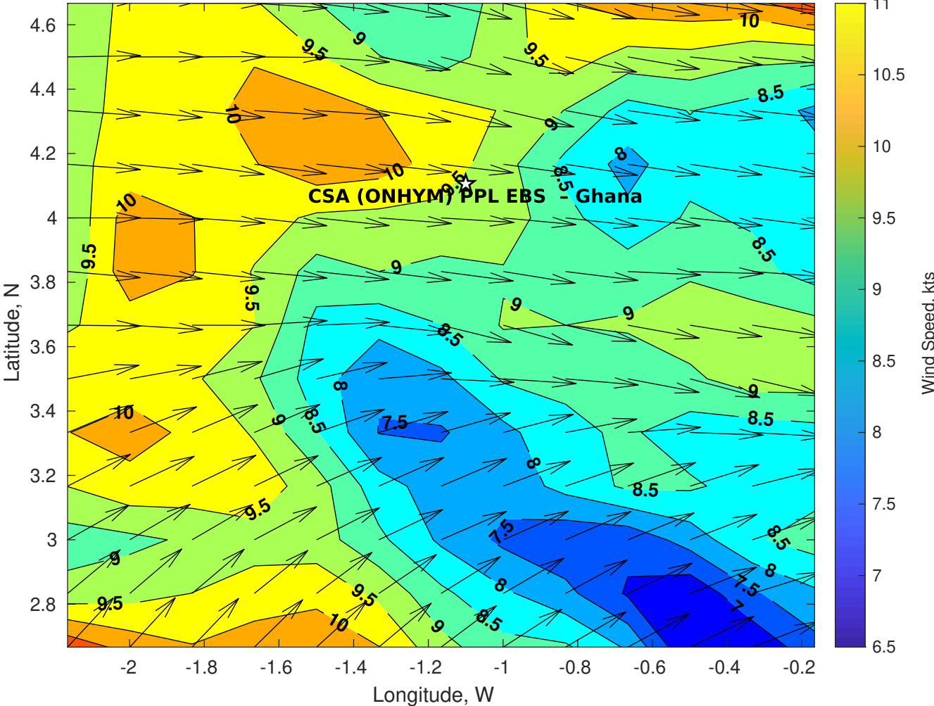
Winds (kts) for CSA (ONHYM) PPL EBS - Ghana at 18-May-2025 09:00:00
