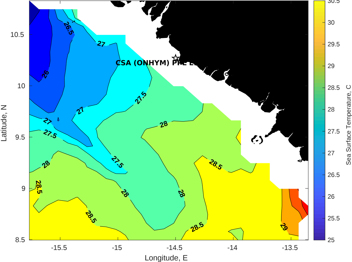
SST for CSA (ONHYM) PPL EBS - Guinea at 17-May-2025 00:00:00
