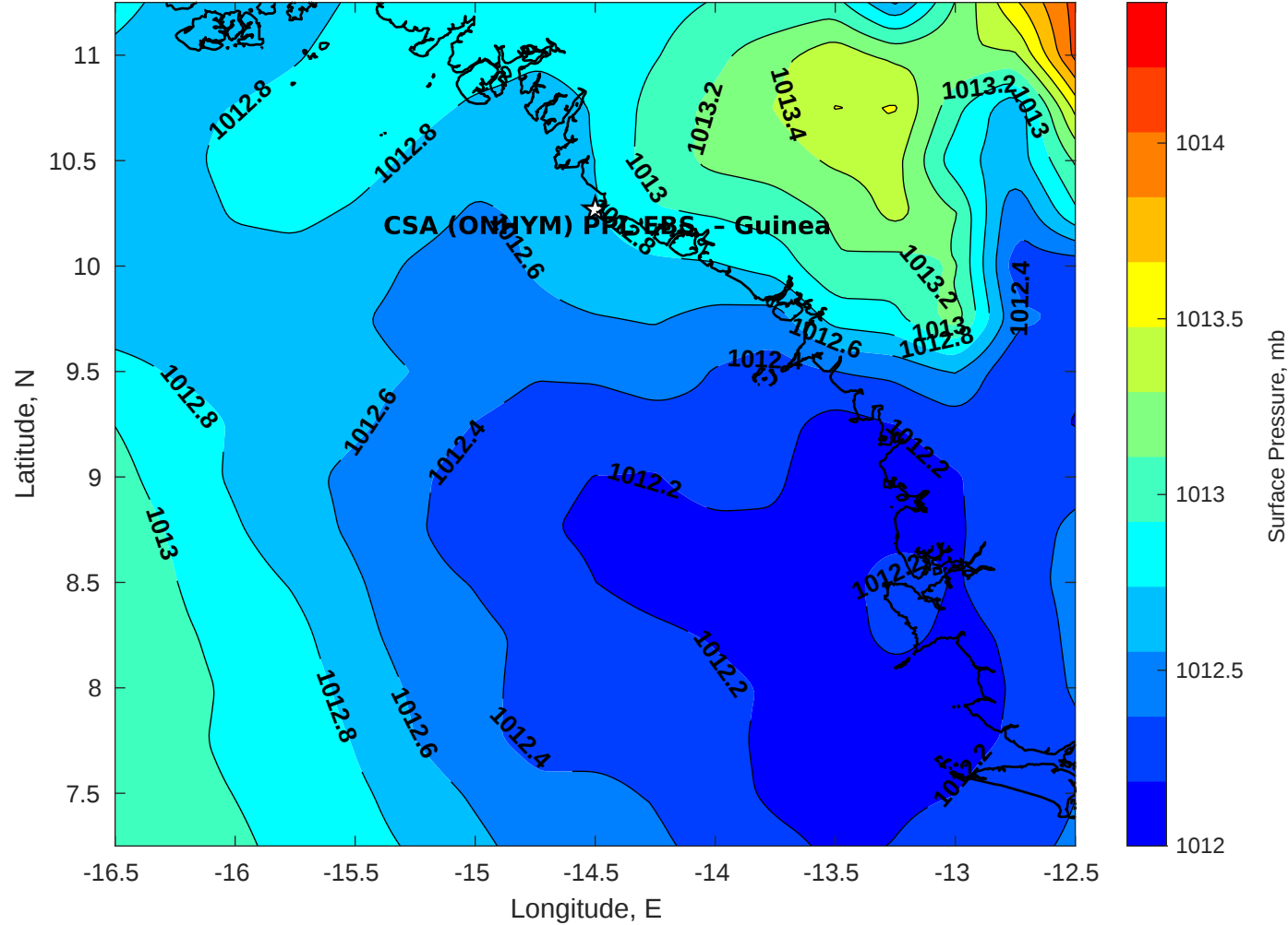
Surface Pressure (mb) for CSA (ONHYM) PPL EBS - Guinea at 20-May-2025 00:00:00
