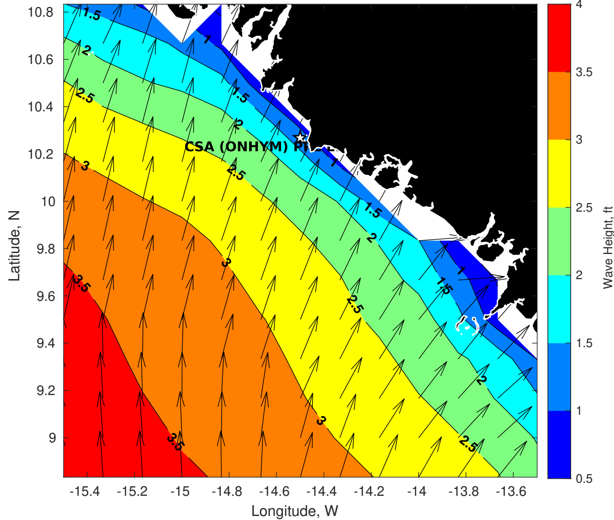
Wave Height (ft) for CSA (ONHYM) PPL EBS - Guinea at 18-May-2025 09:00:00
