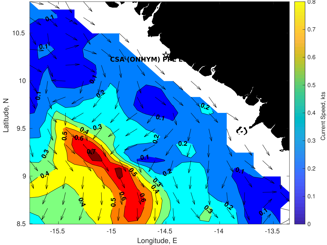
Surface Currents for CSA (ONHYM) PPL EBS - Guinea at 17-May-2025 00:00:00
