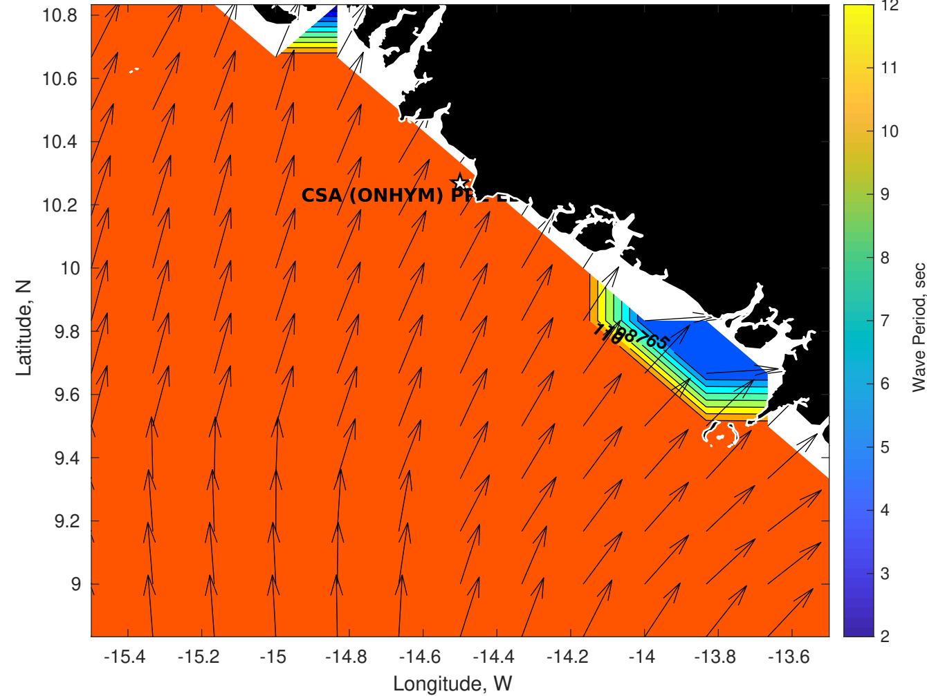
Wave Period (sec) for CSA (ONHYM) PPL EBS - Guinea at 18-May-2025 09:00:00
