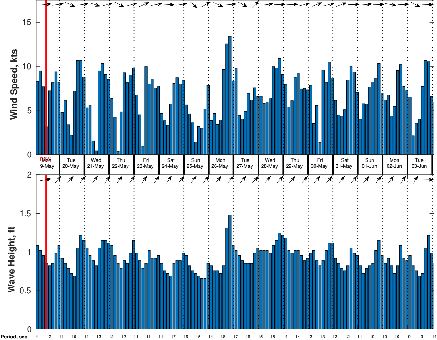
Wind & Wave Forecast for CSA (ONHYM) PPL EBS - Guinea from 18-May-2025 01:00:00 to 03-Jun-2025 01:00:00
