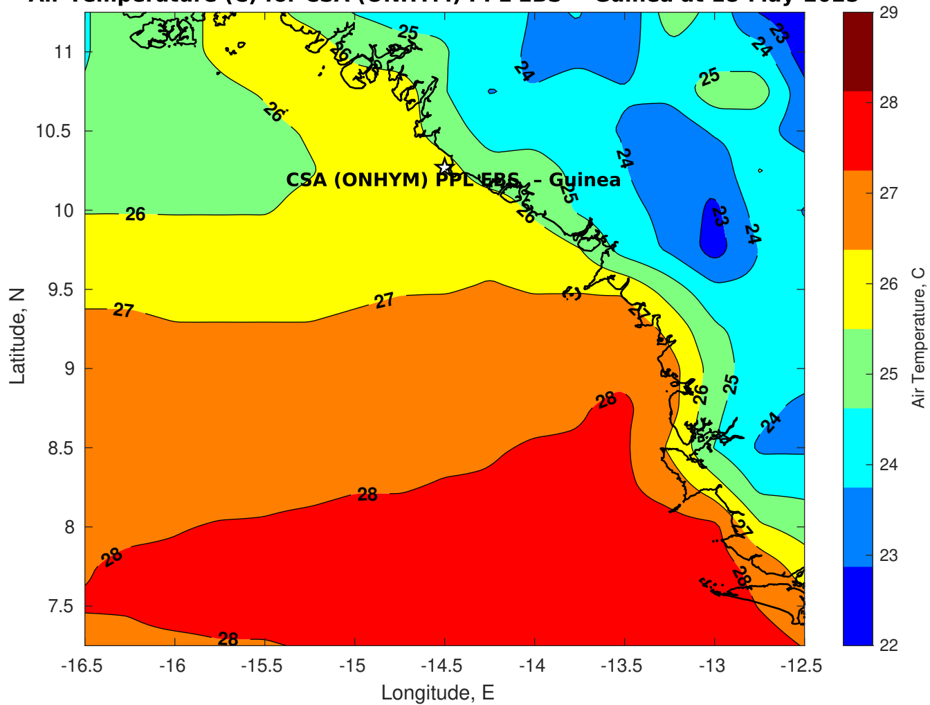
Air Temperature (C) for CSA (ONHYM) PPL EBS - Guinea at 18-May-2025
