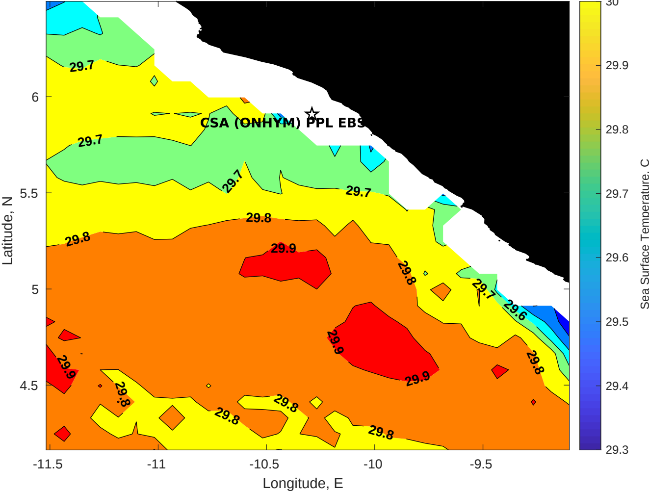
SST for CSA (ONHYM) PPL EBS - Liberia at 17-May-2025 00:00:00
