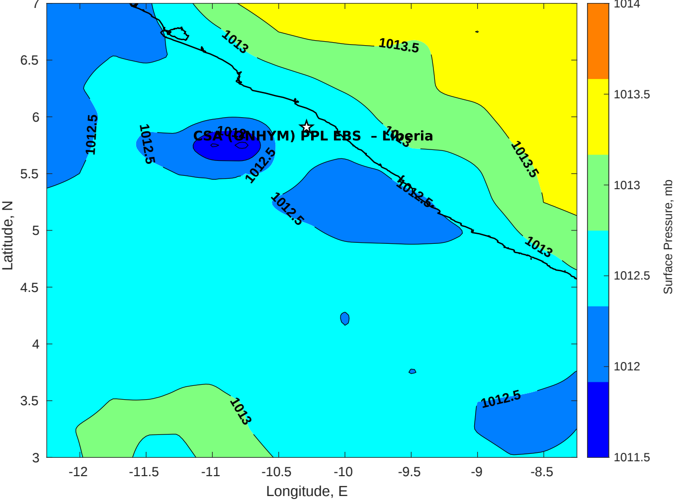
Surface Pressure (mb) for CSA (ONHYM) PPL EBS - Liberia at 18-May-2025 00:00:00
