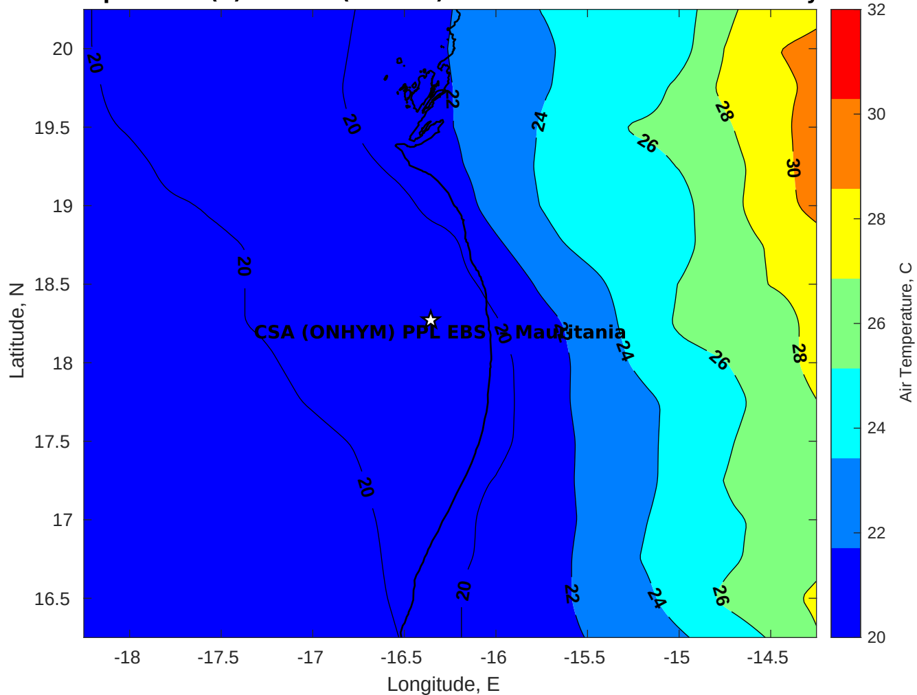
Air Temperature (C) for CSA (ONHYM) PPL EBS - Mauritania at 18-May-2025
