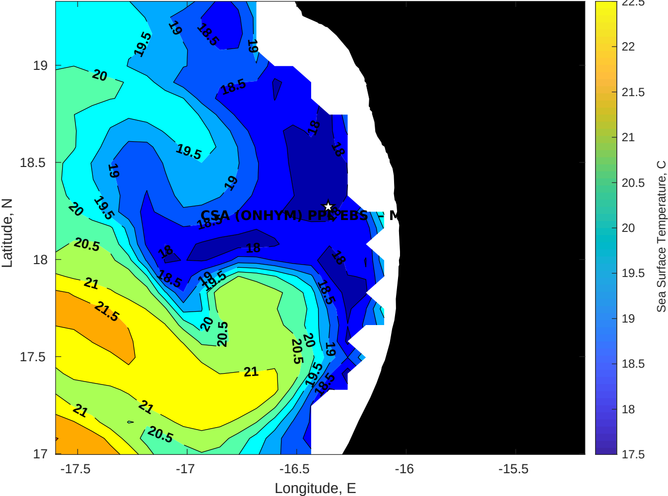
SST for CSA (ONHYM) PPL EBS - Mauritania at 17-May-2025 00:00:00
