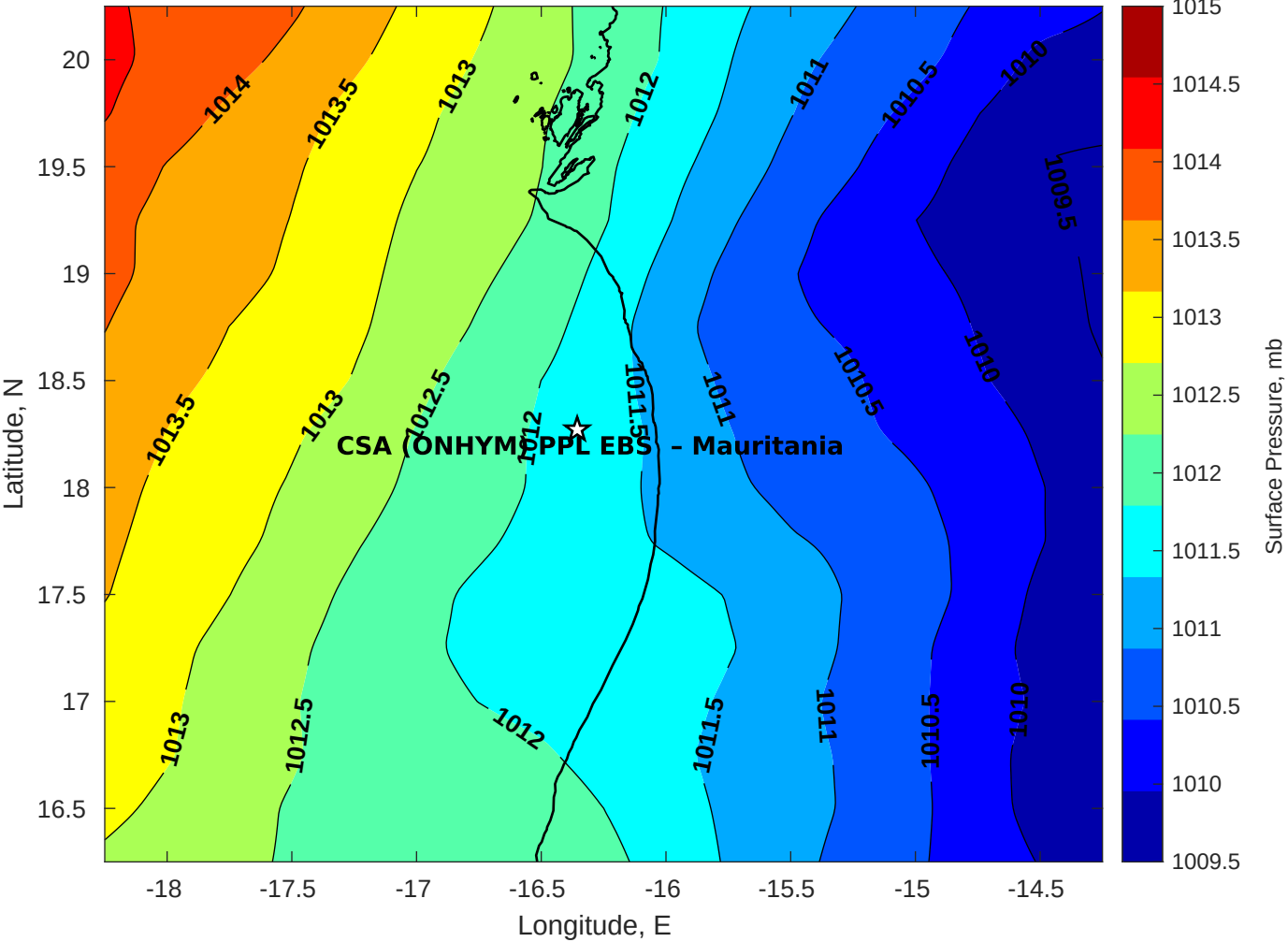
Surface Pressure (mb) for CSA (ONHYM) PPL EBS - Mauritania at 18-May-2025 00:00:00
