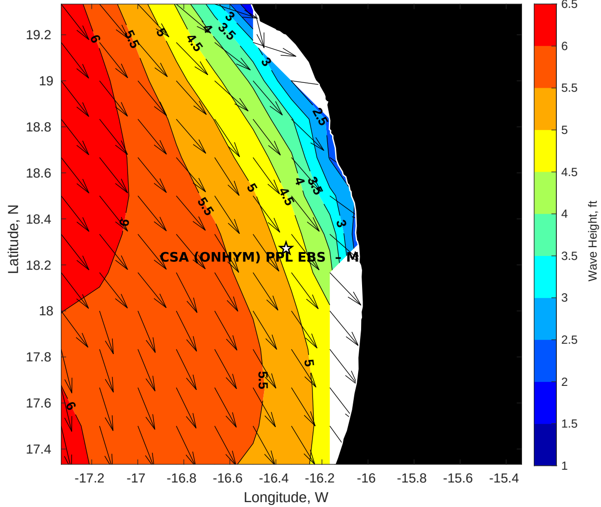
Wave Height (ft) for CSA (ONHYM) PPL EBS - Mauritania at 18-May-2025 09:00:00
