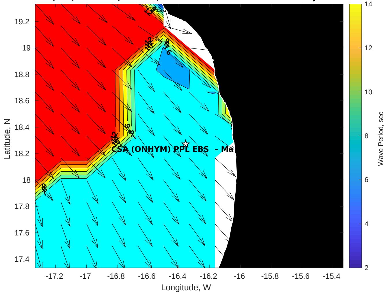
Wave Period (sec) for CSA (ONHYM) PPL EBS - Mauritania at 18-May-2025 09:00:00
