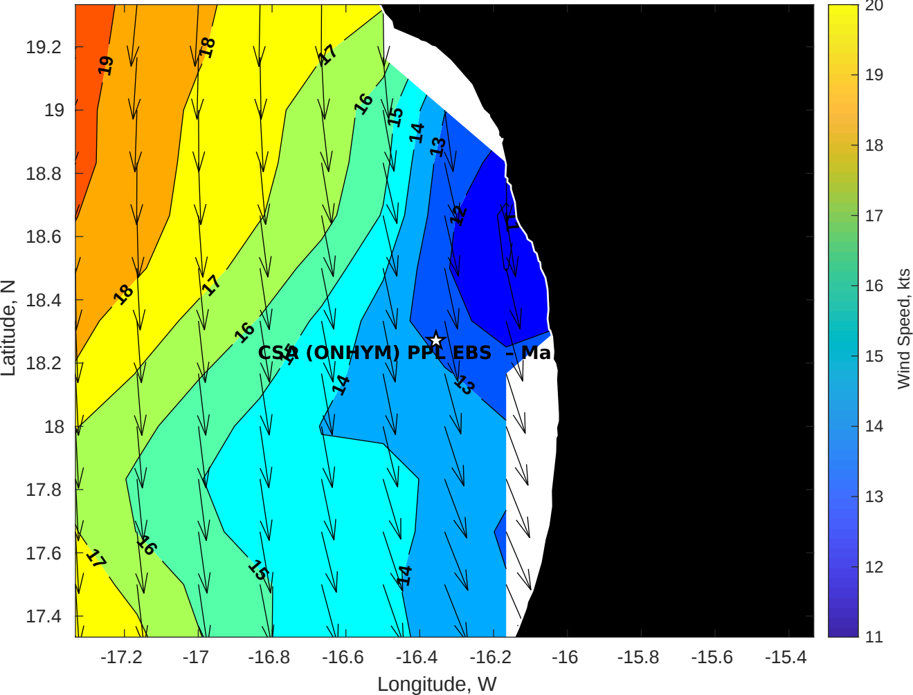
Winds (kts) for CSA (ONHYM) PPL EBS - Mauritania at 18-May-2025 09:00:00
