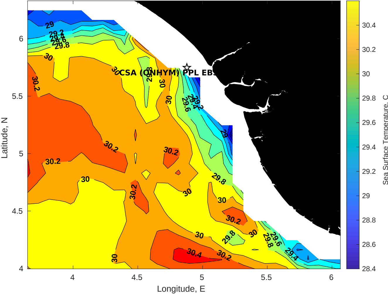
SST for CSA (ONHYM) PPL EBS - Nigeria at 17-May-2025 00:00:00
