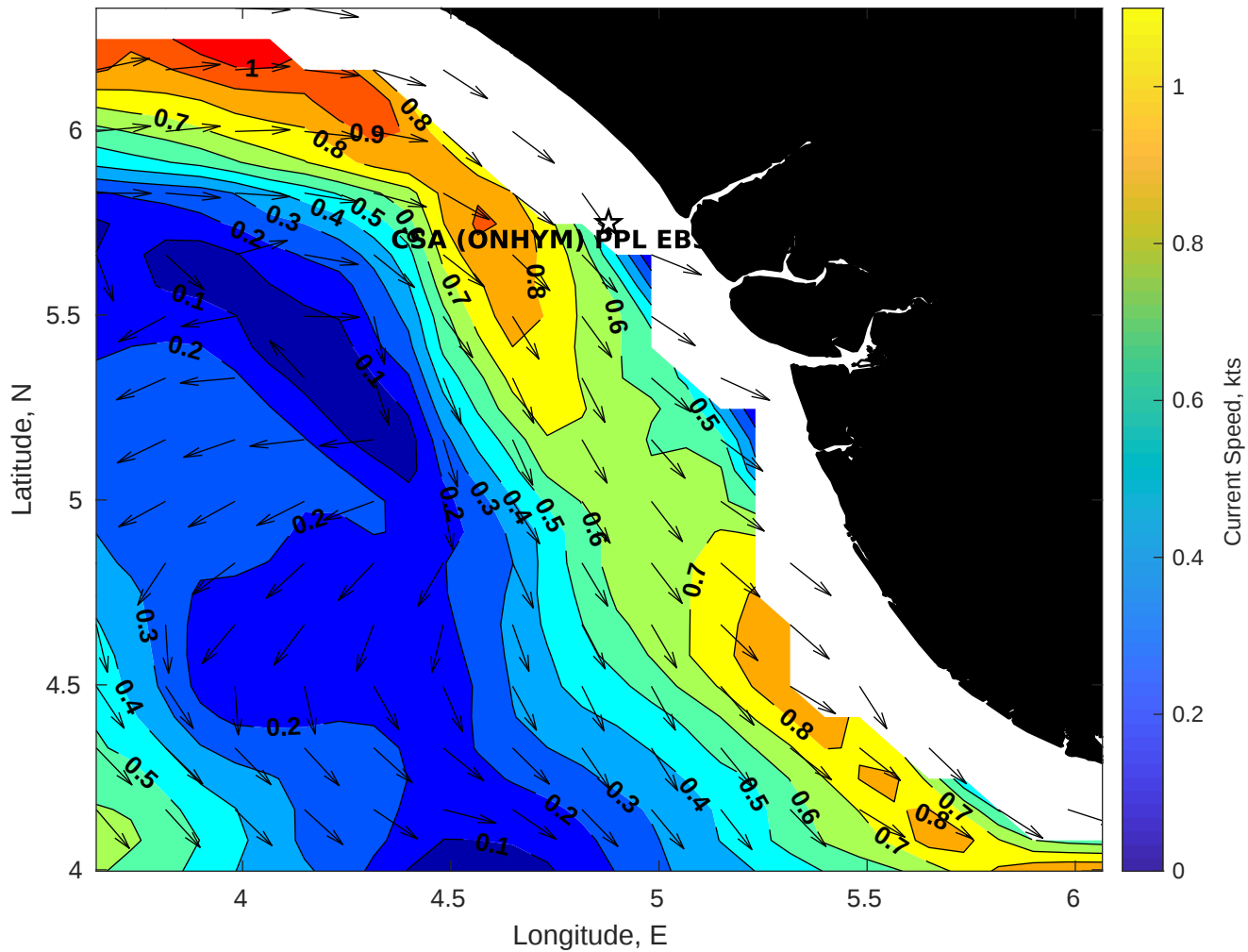
Surface Currents for CSA (ONHYM) PPL EBS - Nigeria at 17-May-2025 00:00:00
