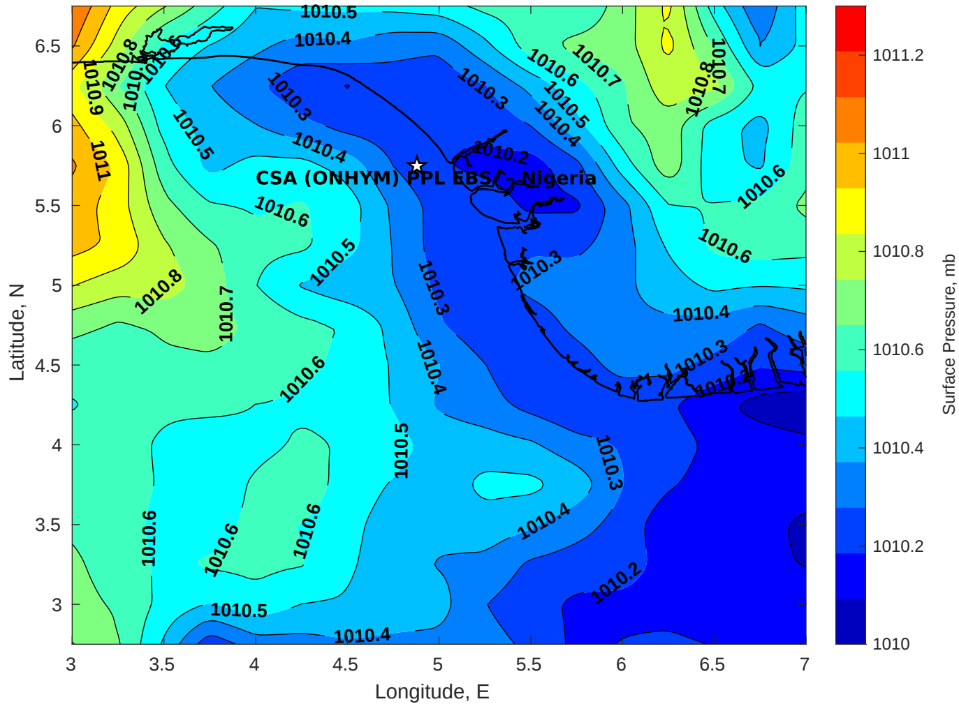
Surface Pressure (mb) for CSA (ONHYM) PPL EBS - Nigeria at 18-May-2025 00:00:00
