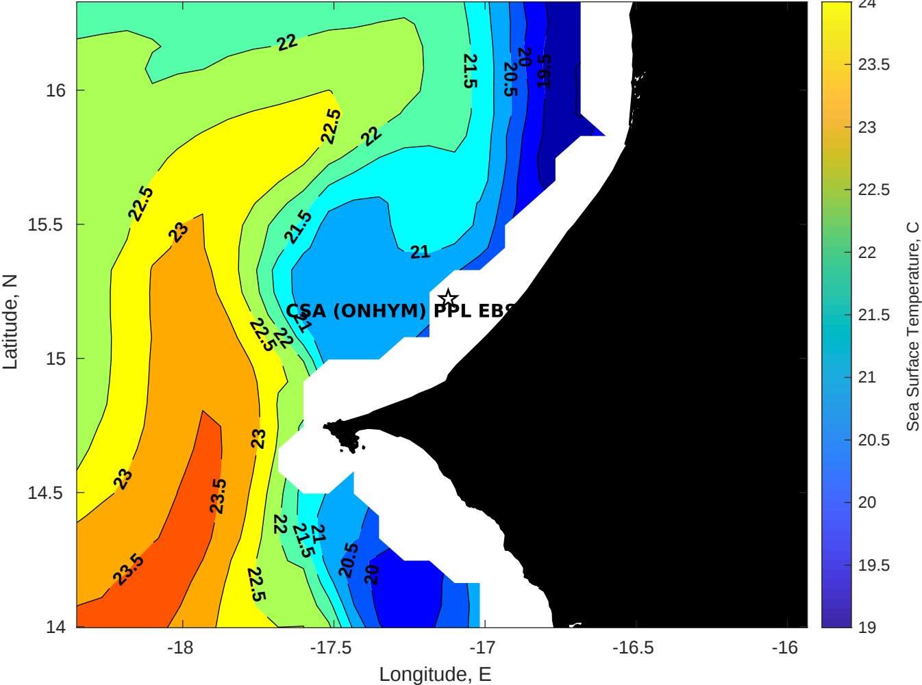
SST for CSA (ONHYM) PPL EBS - Senegal at 17-May-2025 00:00:00
