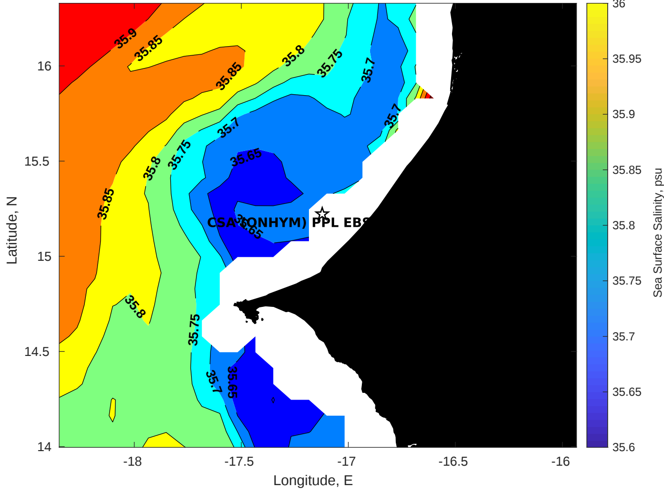
Surface Salinity for CSA (ONHYM) PPL EBS - Senegal at 17-May-2025 00:00:00
