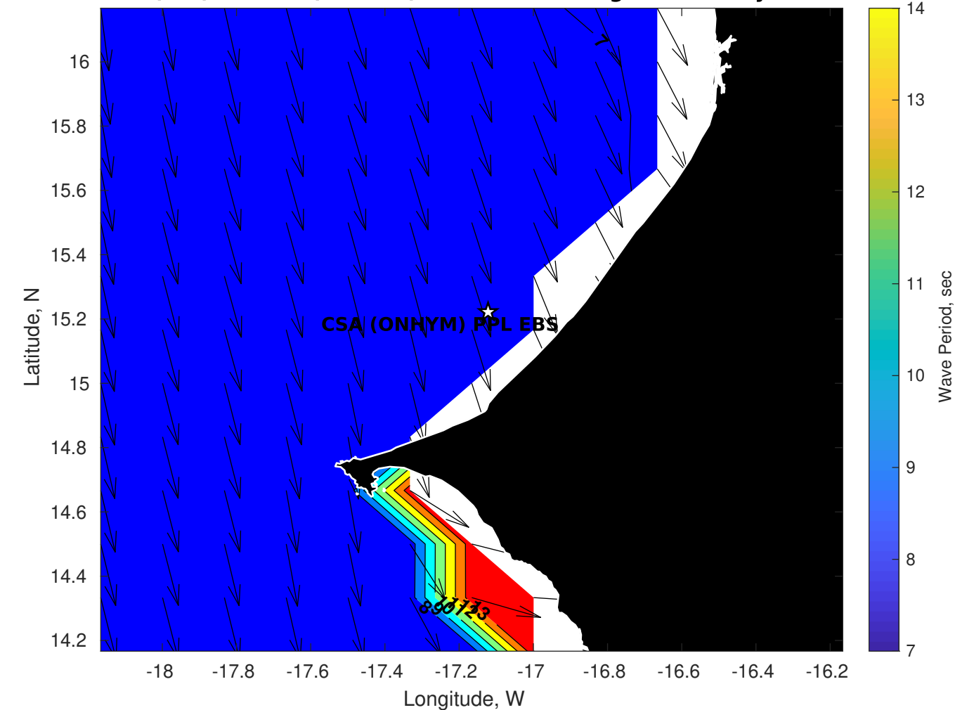
Wave Period (sec) for CSA (ONHYM) PPL EBS - Senegal at 18-May-2025 09:00:00
