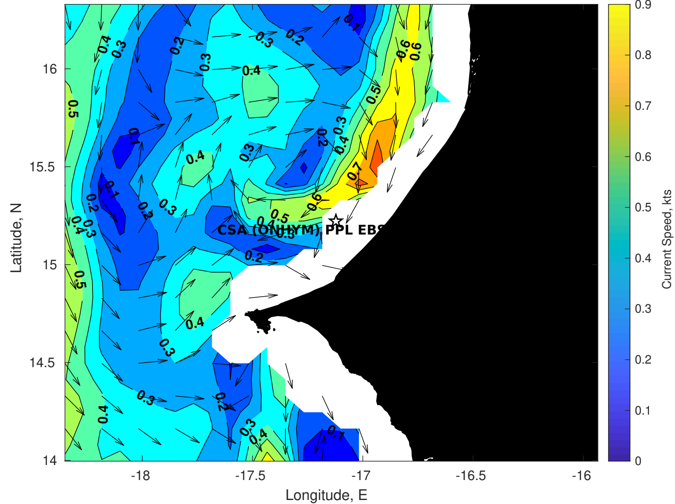
Surface Currents for CSA (ONHYM) PPL EBS - Senegal at 17-May-2025 00:00:00
