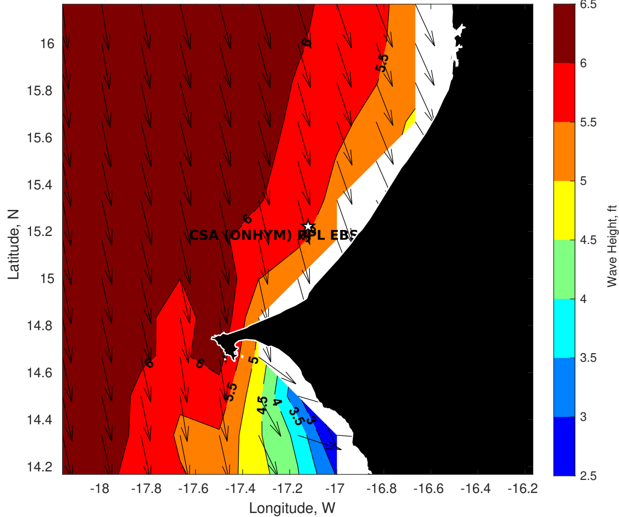
Wave Height (ft) for CSA (ONHYM) PPL EBS - Senegal at 18-May-2025 09:00:00
