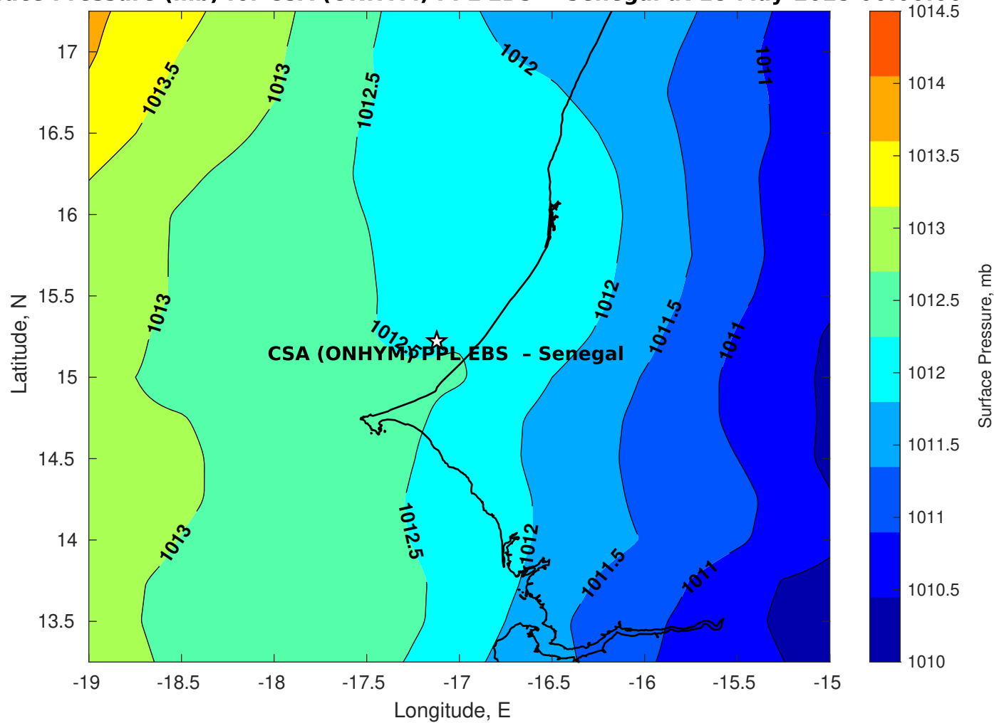
Surface Pressure (mb) for CSA (ONHYM) PPL EBS - Senegal at 18-May-2025 00:00:00
