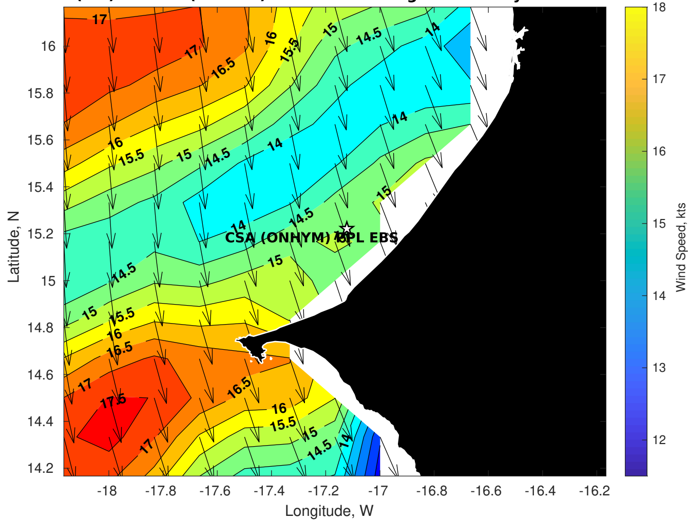
Winds (kts) for CSA (ONHYM) PPL EBS - Senegal at 18-May-2025 09:00:00
