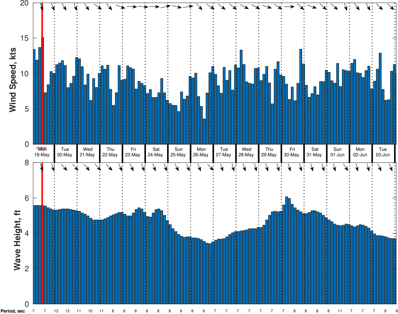
Wind & Wave Forecast for CSA (ONHYM) PPL EBS - Senegal from 18-May-2025 01:00:00 to 03-Jun-2025 01:00:00
