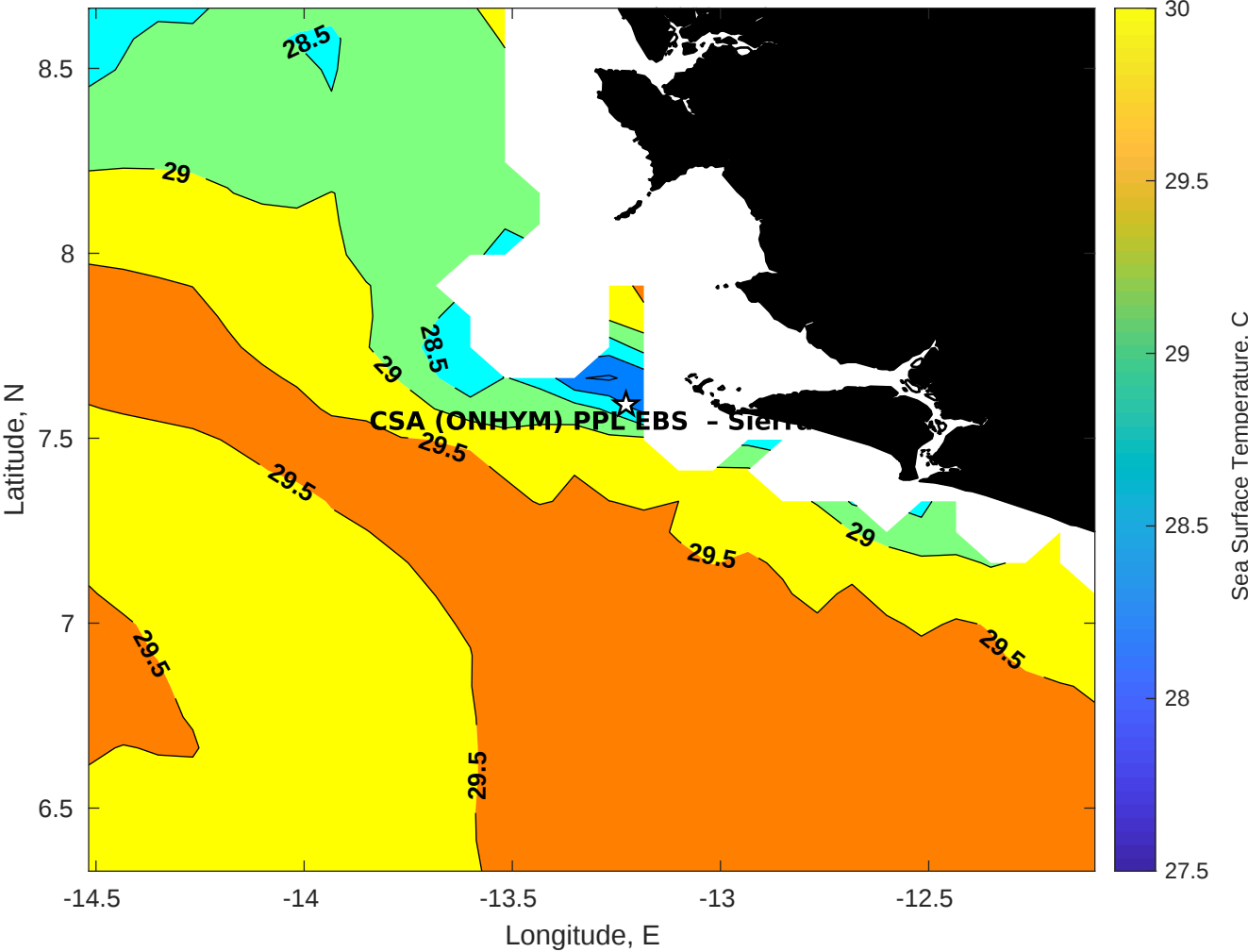
SST for CSA (ONHYM) PPL EBS - Sierra Leone at 17-May-2025 00:00:00
