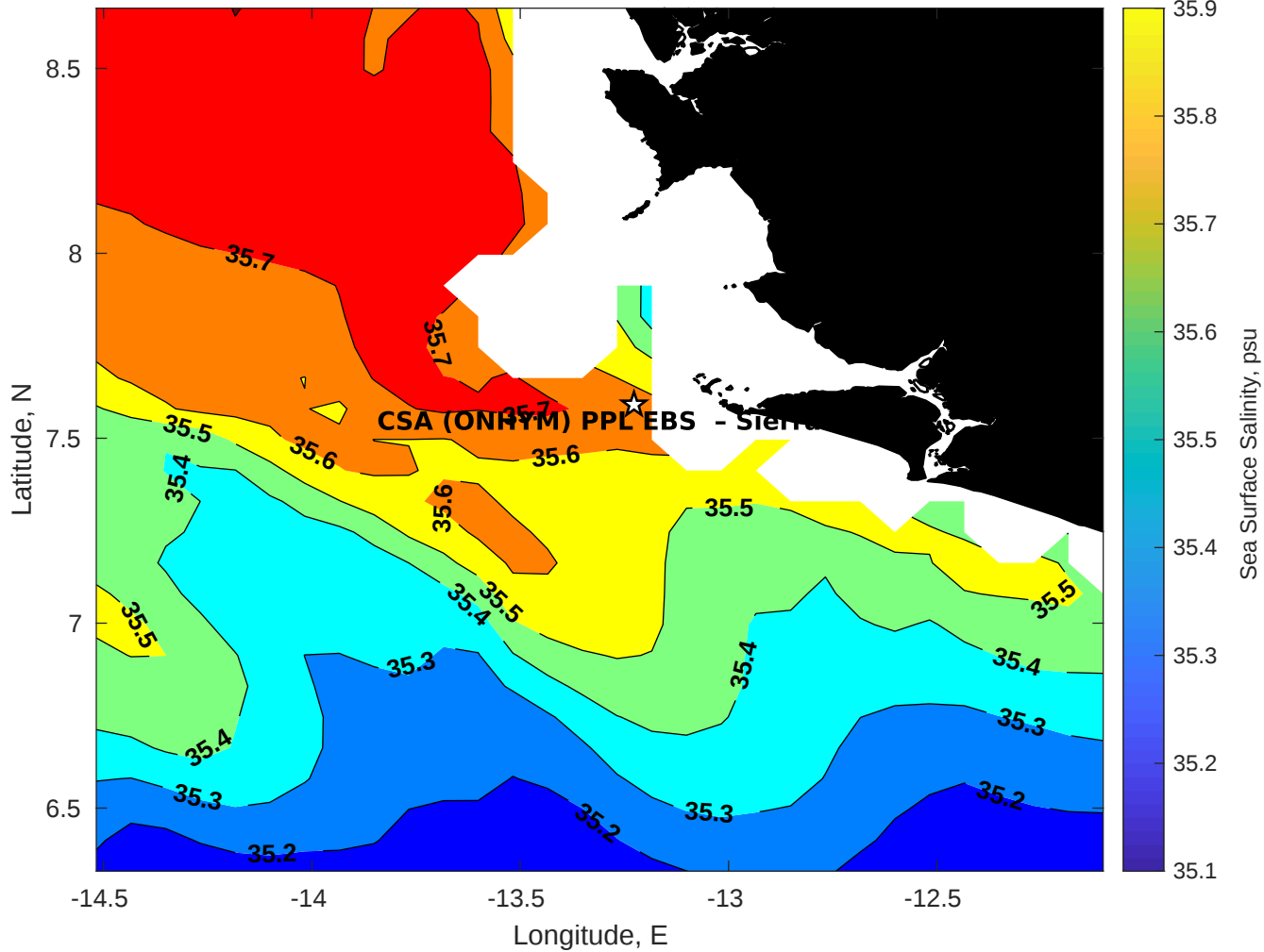
Surface Salinity for CSA (ONHYM) PPL EBS - Sierra Leone at 17-May-2025 00:00:00
