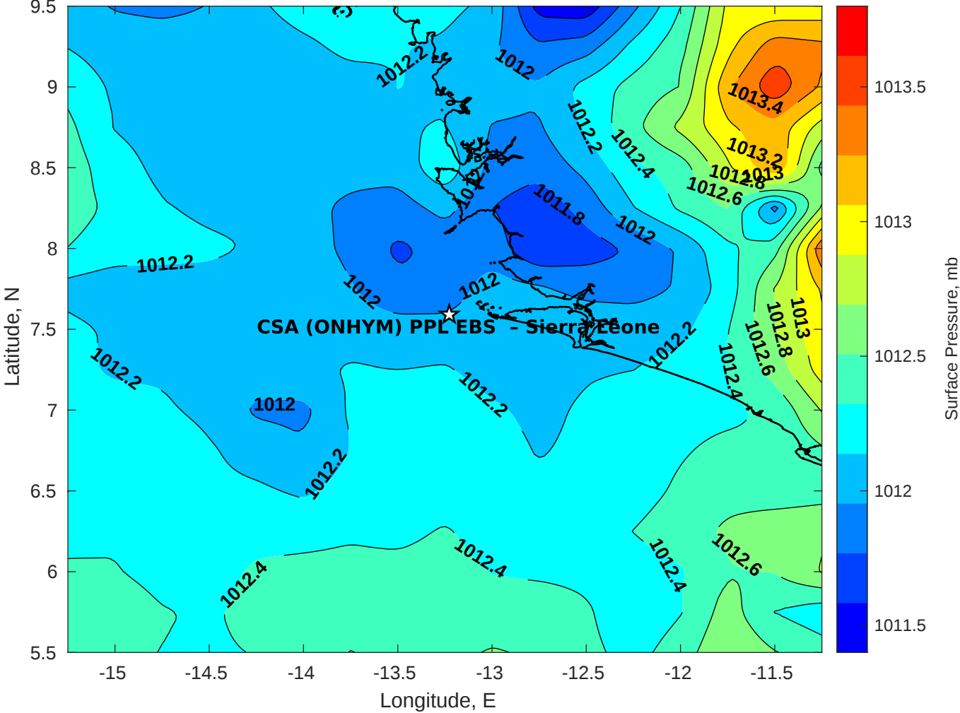
Surface Pressure (mb) for CSA (ONHYM) PPL EBS - Sierra Leone at 18-May-2025 00:00:00
