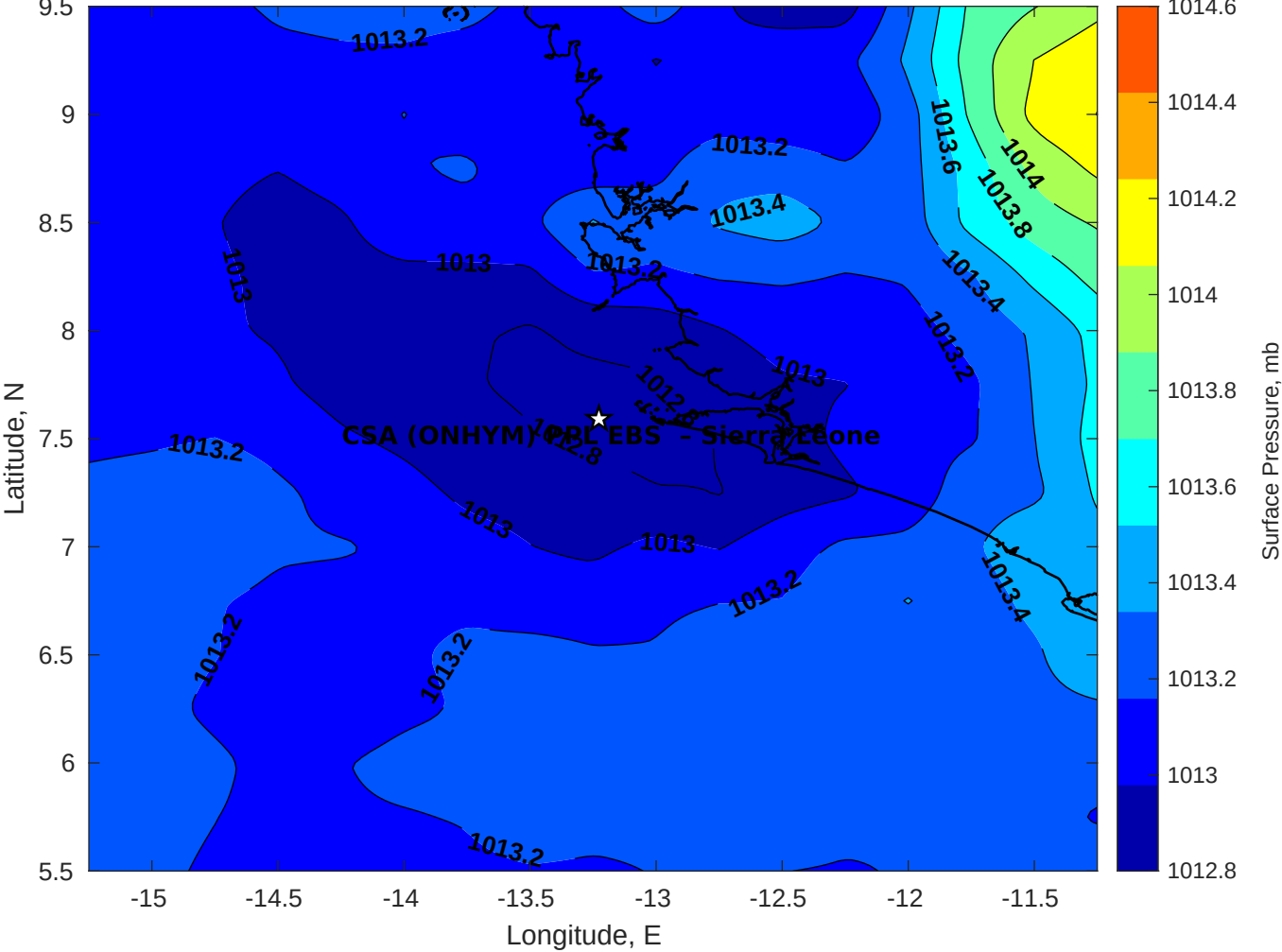
Surface Pressure (mb) for CSA (ONHYM) PPL EBS - Sierra Leone at 19-May-2025 00:00:00
