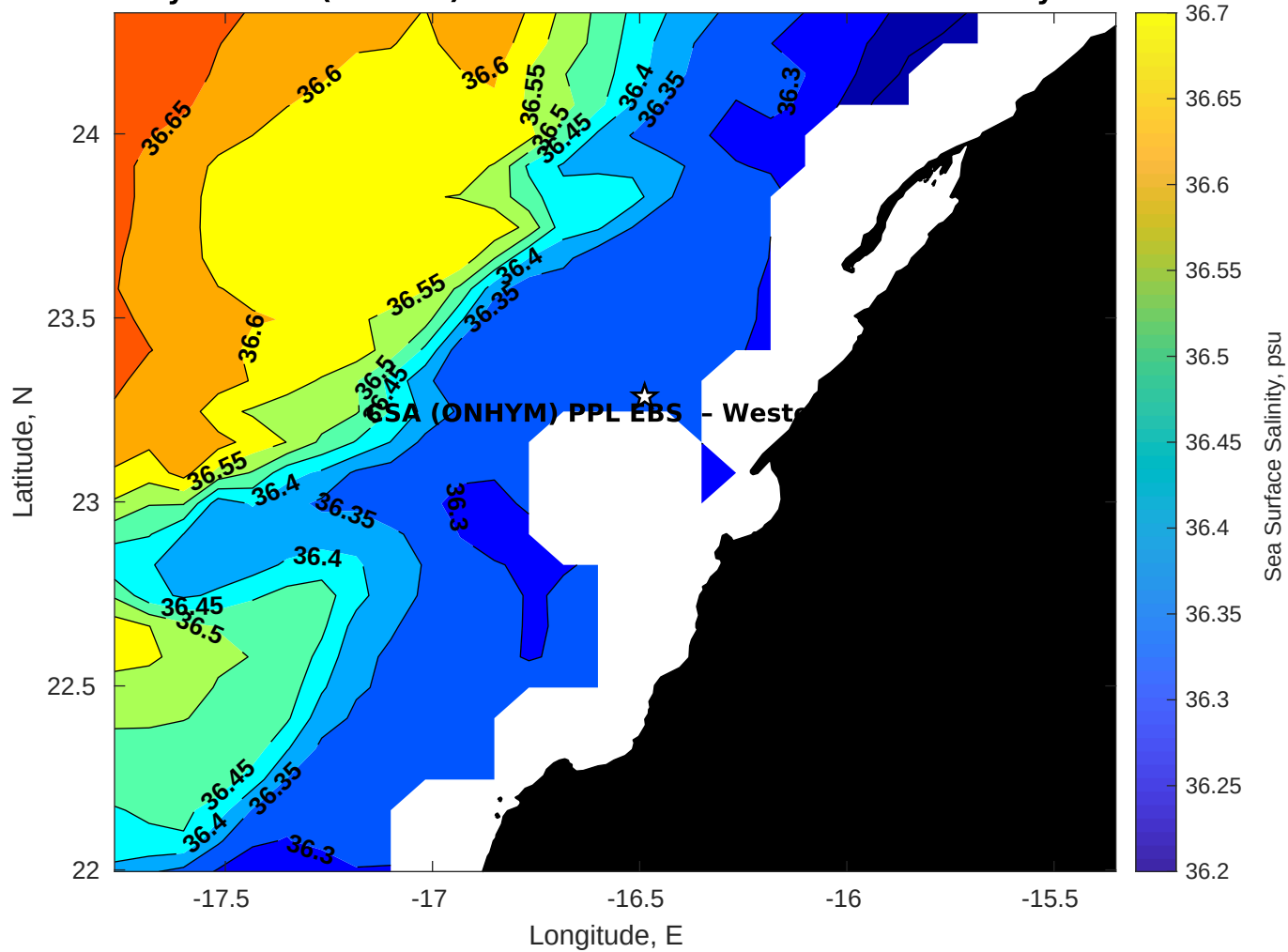
Surface Salinity for CSA (ONHYM) PPL EBS - Western Sahara at 17-May-2025 00:00:00
